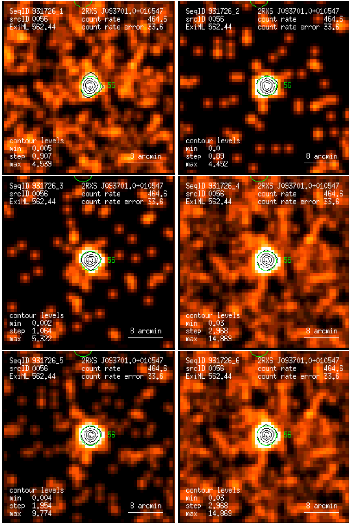
Figure 56: RASS 931726: detection 0056: band rate images, Gaussian filter: (1) PSPC channels 11 – 41, (2) 52 – 90, (3) 91 – 201, (4) 11 – 235, (5) 52 – 201, (6) 11 – 201. Broad band rates in counts/ks. Band rate contour levels in counts/ks/arcmin 2 .
