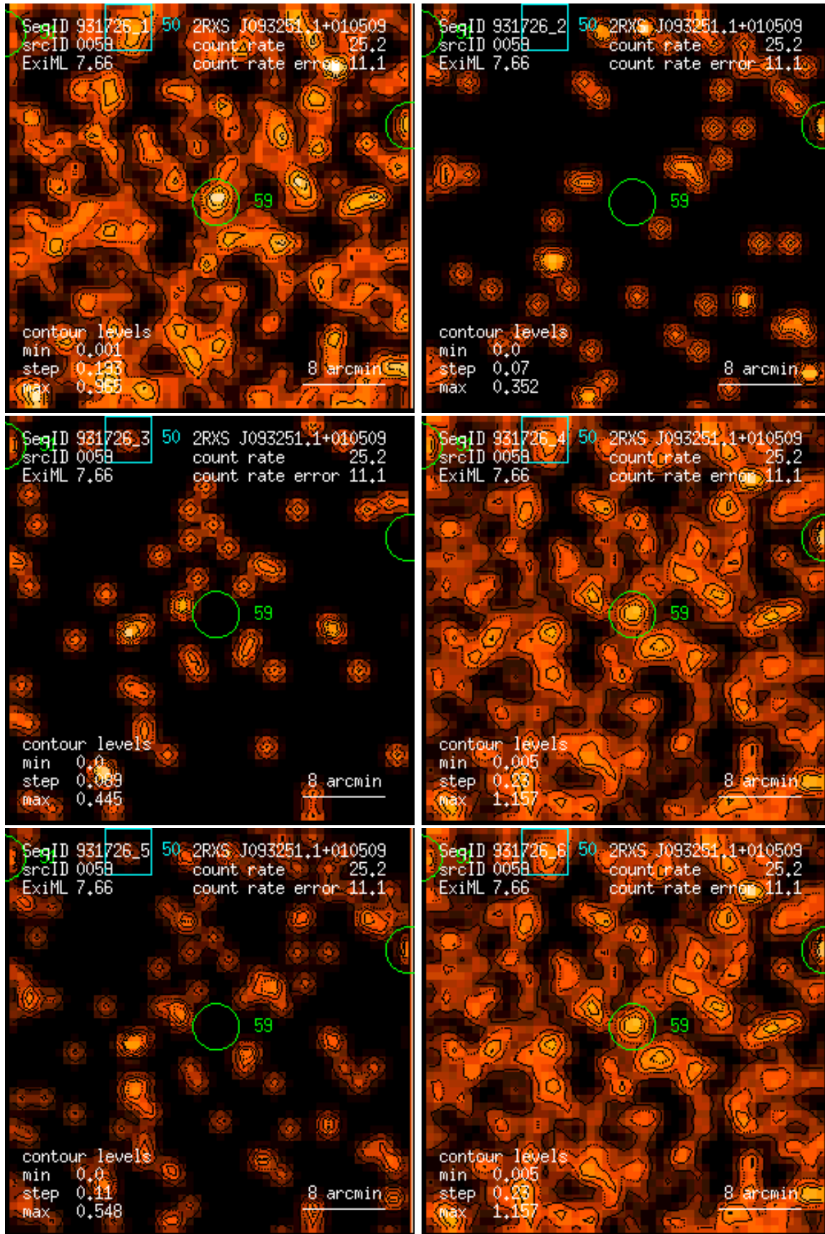
Figure 59: RASS 931726: detection 0059: band rate images, Gaussian filter: (1) PSPC channels 11 – 41, (2) 52 – 90, (3) 91 – 201, (4) 11 – 235, (5) 52 – 201, (6) 11 – 201. Broad band rates in counts/ks. Band rate contour levels in counts/ks/arcmin 2 .
