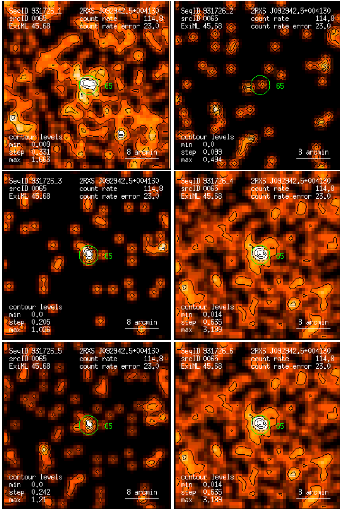
Figure 65: RASS 931726: detection 0065: band rate images, Gaussian filter: (1) PSPC channels 11 – 41, (2) 52 – 90, (3) 91 – 201, (4) 11 – 235, (5) 52 – 201, (6) 11 – 201. Broad band rates in counts/ks. Band rate contour levels in counts/ks/arcmin 2 .
