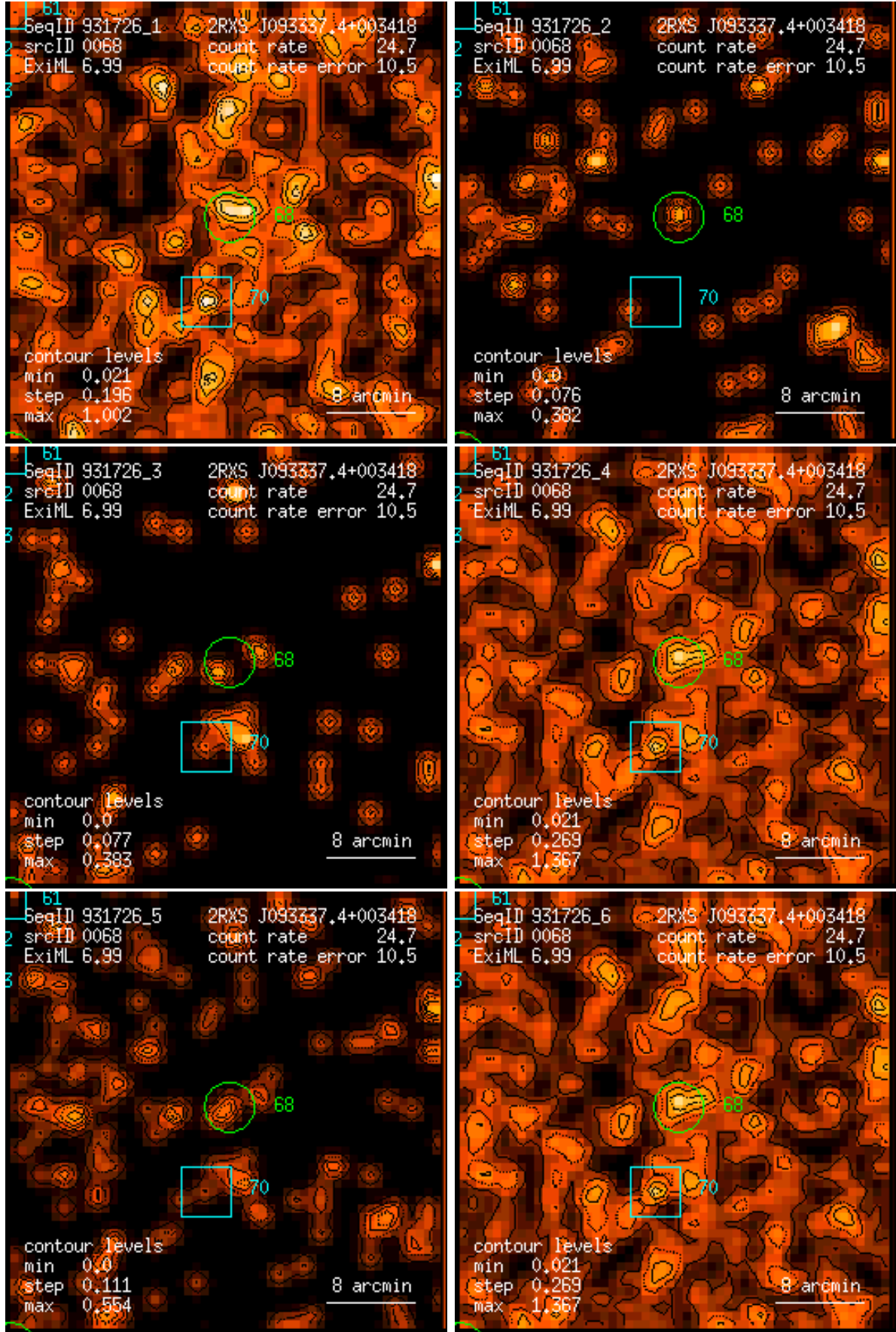
Figure 68: RASS 931726: detection 0068: band rate images, Gaussian filter: (1) PSPC channels 11 – 41, (2) 52 – 90, (3) 91 – 201, (4) 11 – 235, (5) 52 – 201, (6) 11 – 201. Broad band rates in counts/ks. Band rate contour levels in counts/ks/arcmin 2 .
