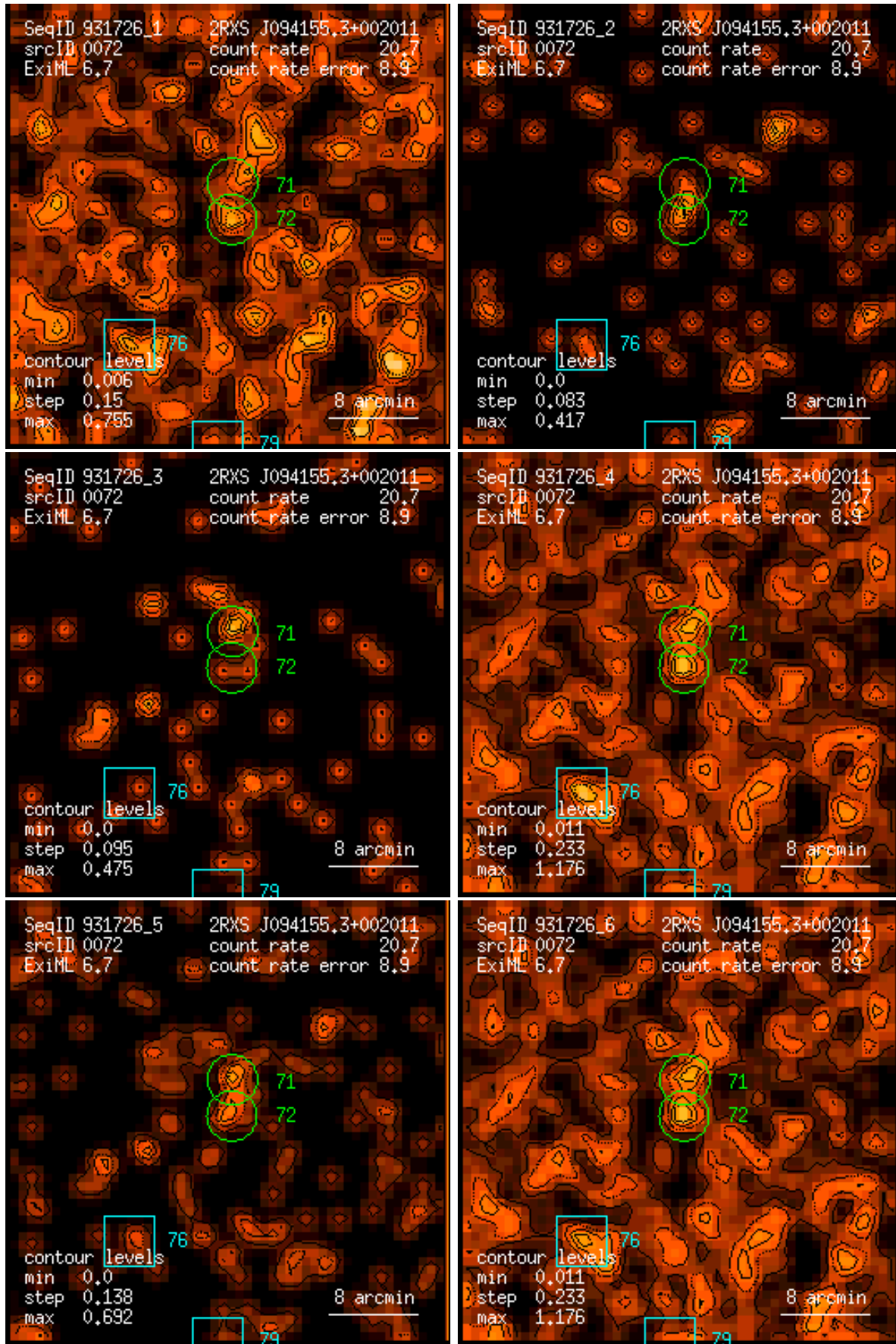
Figure 72: RASS 931726: detection 0072: band rate images, Gaussian filter: (1) PSPC channels 11 – 41, (2) 52 – 90, (3) 91 – 201, (4) 11 – 235, (5) 52 – 201, (6) 11 – 201. Broad band rates in counts/ks. Band rate contour levels in counts/ks/arcmin 2 .
