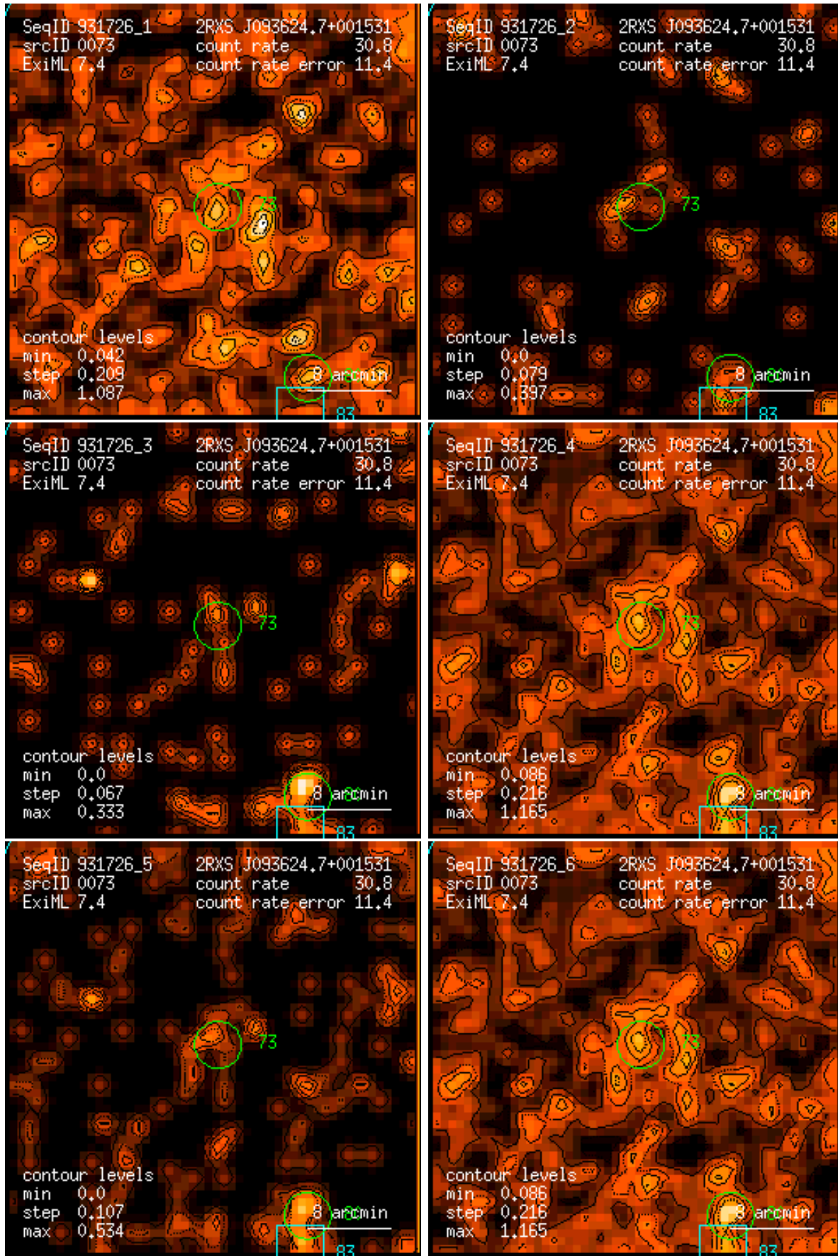
Figure 73: RASS 931726: detection 0073: band rate images, Gaussian filter: (1) PSPC channels 11 – 41, (2) 52 – 90, (3) 91 – 201, (4) 11 – 235, (5) 52 – 201, (6) 11 – 201. Broad band rates in counts/ks. Band rate contour levels in counts/ks/arcmin 2 .
