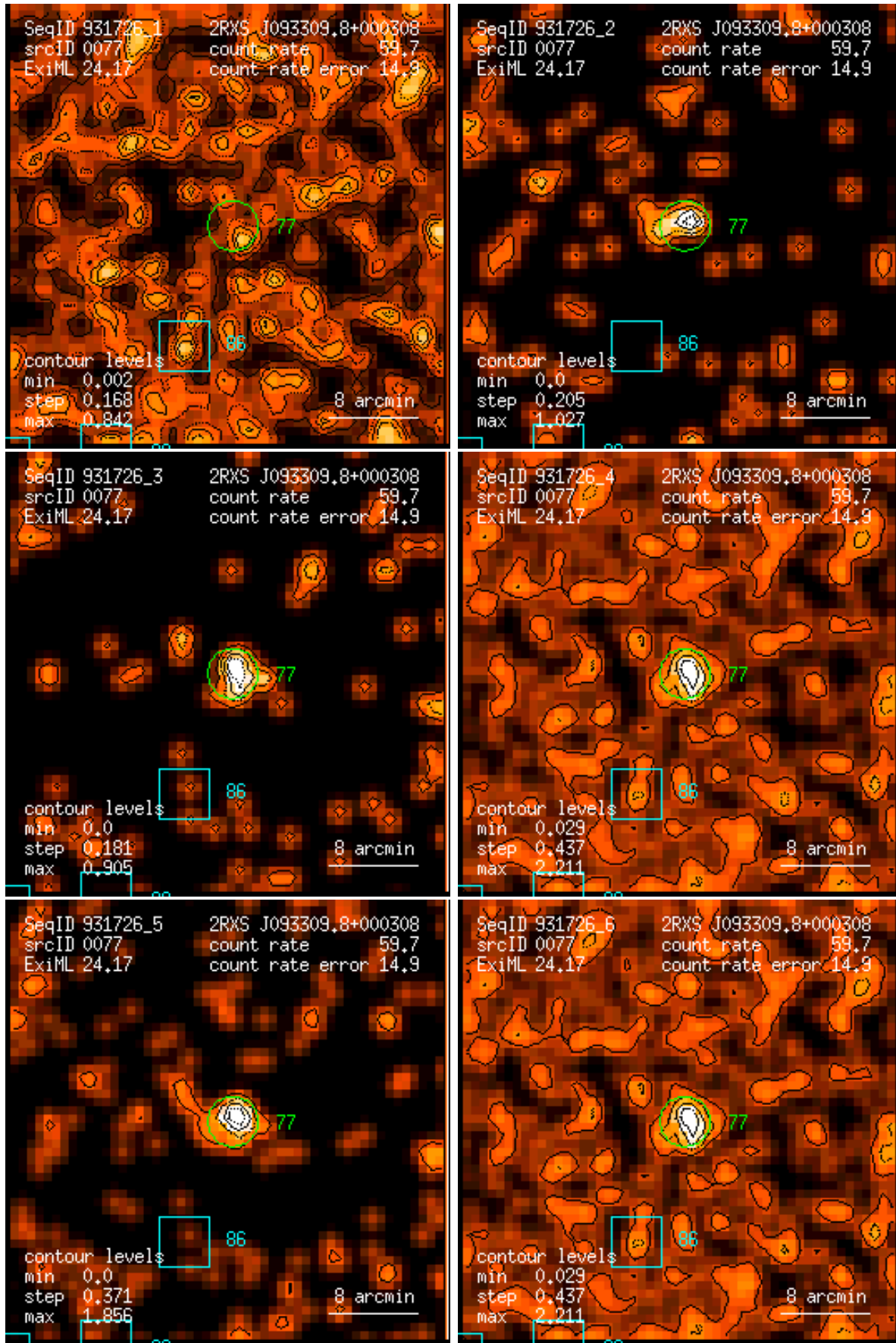
Figure 77: RASS 931726: detection 0077: band rate images, Gaussian filter: (1) PSPC channels 11 – 41, (2) 52 – 90, (3) 91 – 201, (4) 11 – 235, (5) 52 – 201, (6) 11 – 201. Broad band rates in counts/ks. Band rate contour levels in counts/ks/arcmin 2 .
