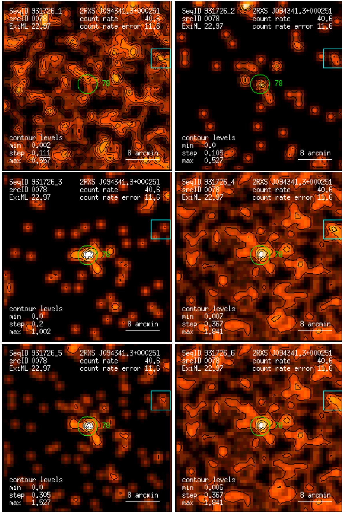
Figure 78: RASS 931726: detection 0078: band rate images, Gaussian filter: (1) PSPC channels 11 – 41, (2) 52 – 90, (3) 91 – 201, (4) 11 – 235, (5) 52 – 201, (6) 11 – 201. Broad band rates in counts/ks. Band rate contour levels in counts/ks/arcmin 2 .
