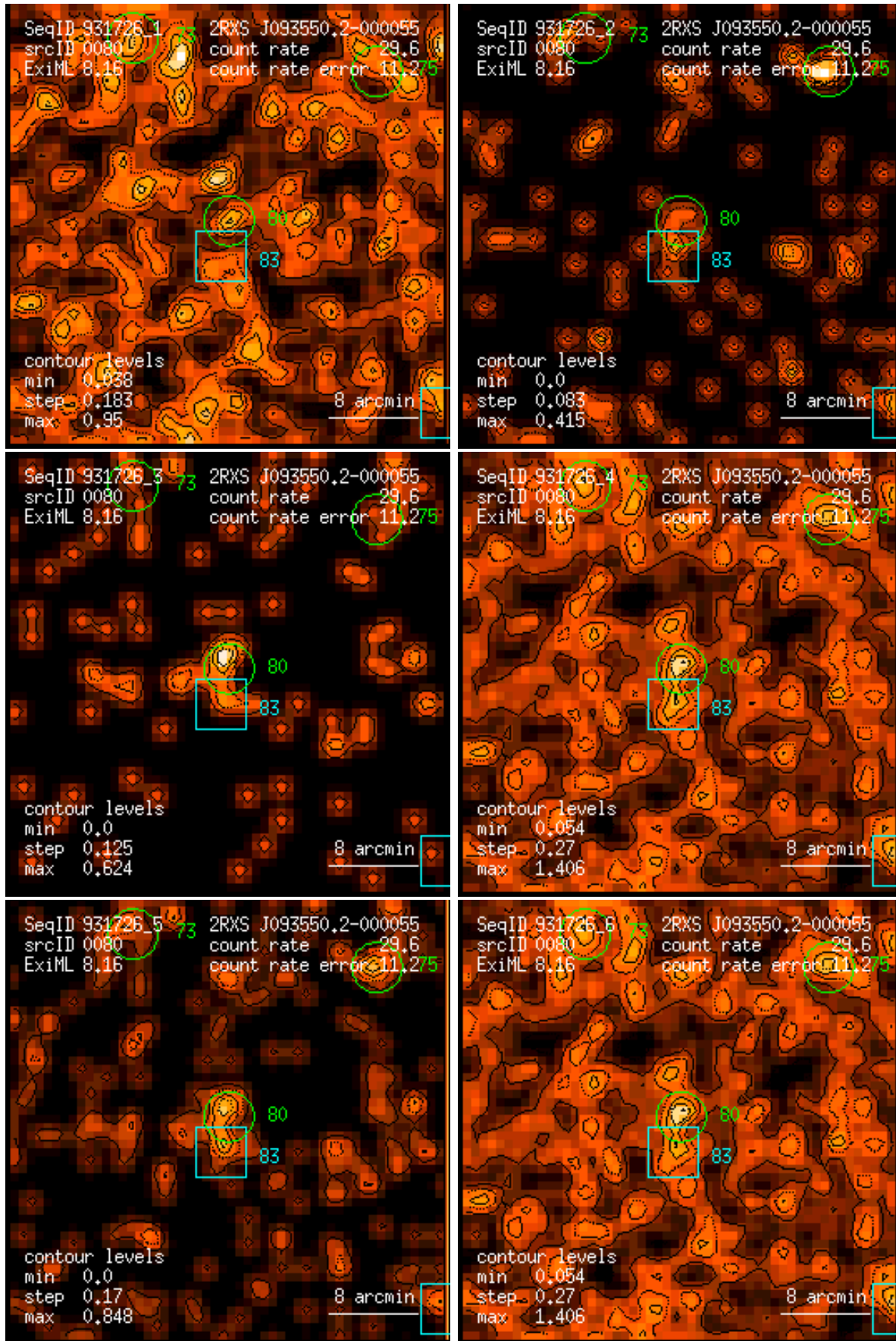
Figure 80: RASS 931726: detection 0080: band rate images, Gaussian filter: (1) PSPC channels 11 – 41, (2) 52 – 90, (3) 91 – 201, (4) 11 – 235, (5) 52 – 201, (6) 11 – 201. Broad band rates in counts/ks. Band rate contour levels in counts/ks/arcmin 2 .
