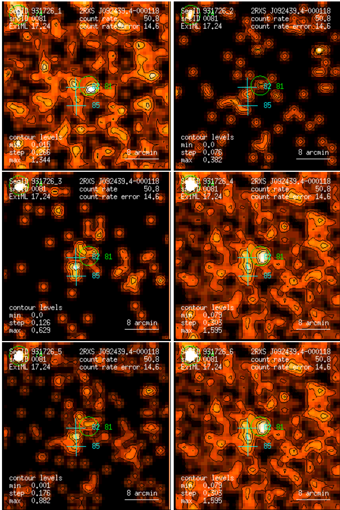
Figure 81: RASS 931726: detection 0081: band rate images, Gaussian filter: (1) PSPC channels 11 – 41, (2) 52 – 90, (3) 91 – 201, (4) 11 – 235, (5) 52 – 201, (6) 11 – 201. Broad band rates in counts/ks. Band rate contour levels in counts/ks/arcmin 2 .
