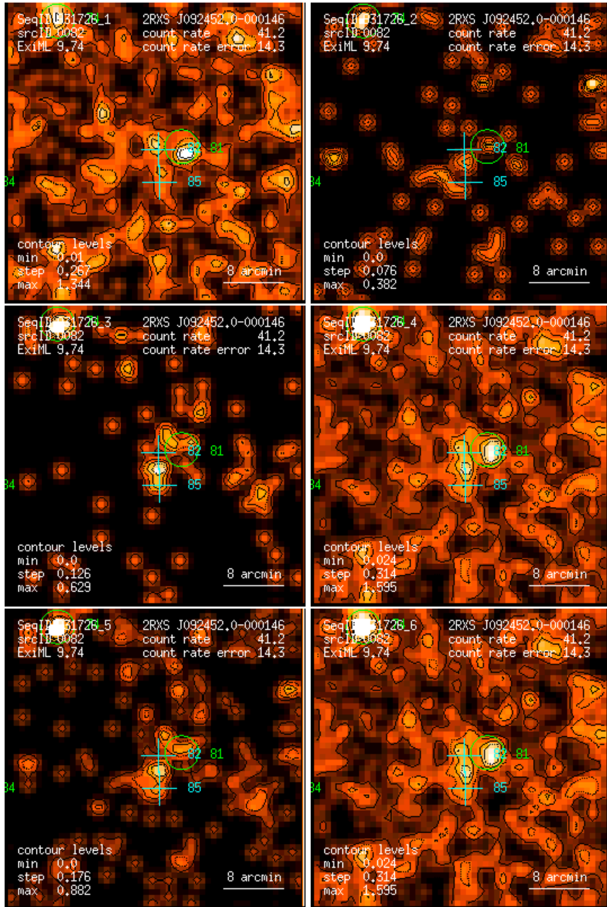
Figure 82: RASS 931726: detection 0082: band rate images, Gaussian filter: (1) PSPC channels 11 – 41, (2) 52 – 90, (3) 91 – 201, (4) 11 – 235, (5) 52 – 201, (6) 11 – 201. Broad band rates in counts/ks. Band rate contour levels in counts/ks/arcmin 2 .
