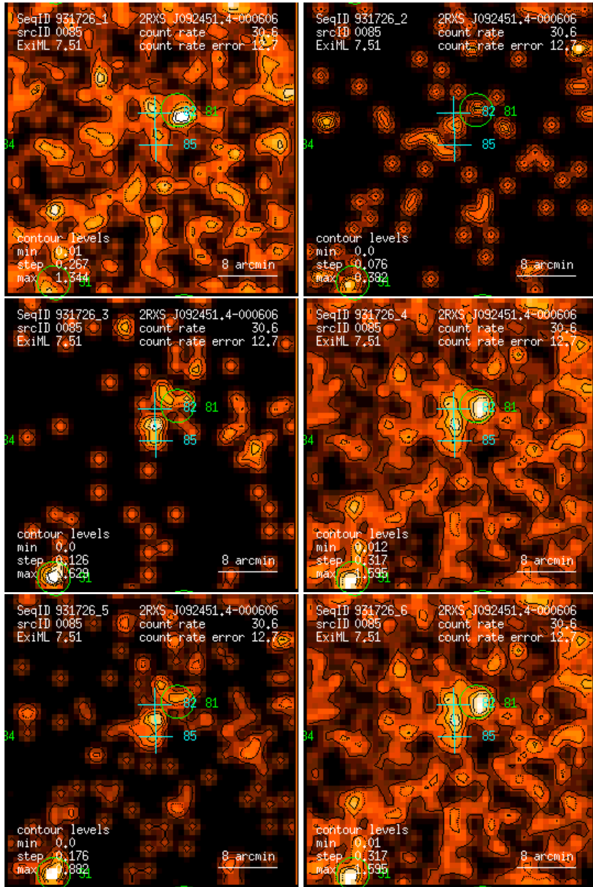
Figure 85: RASS 931726: detection 0085: band rate images, Gaussian filter: (1) PSPC channels 11 – 41, (2) 52 – 90, (3) 91 – 201, (4) 11 – 235, (5) 52 – 201, (6) 11 – 201. Broad band rates in counts/ks. Band rate contour levels in counts/ks/arcmin 2 .
