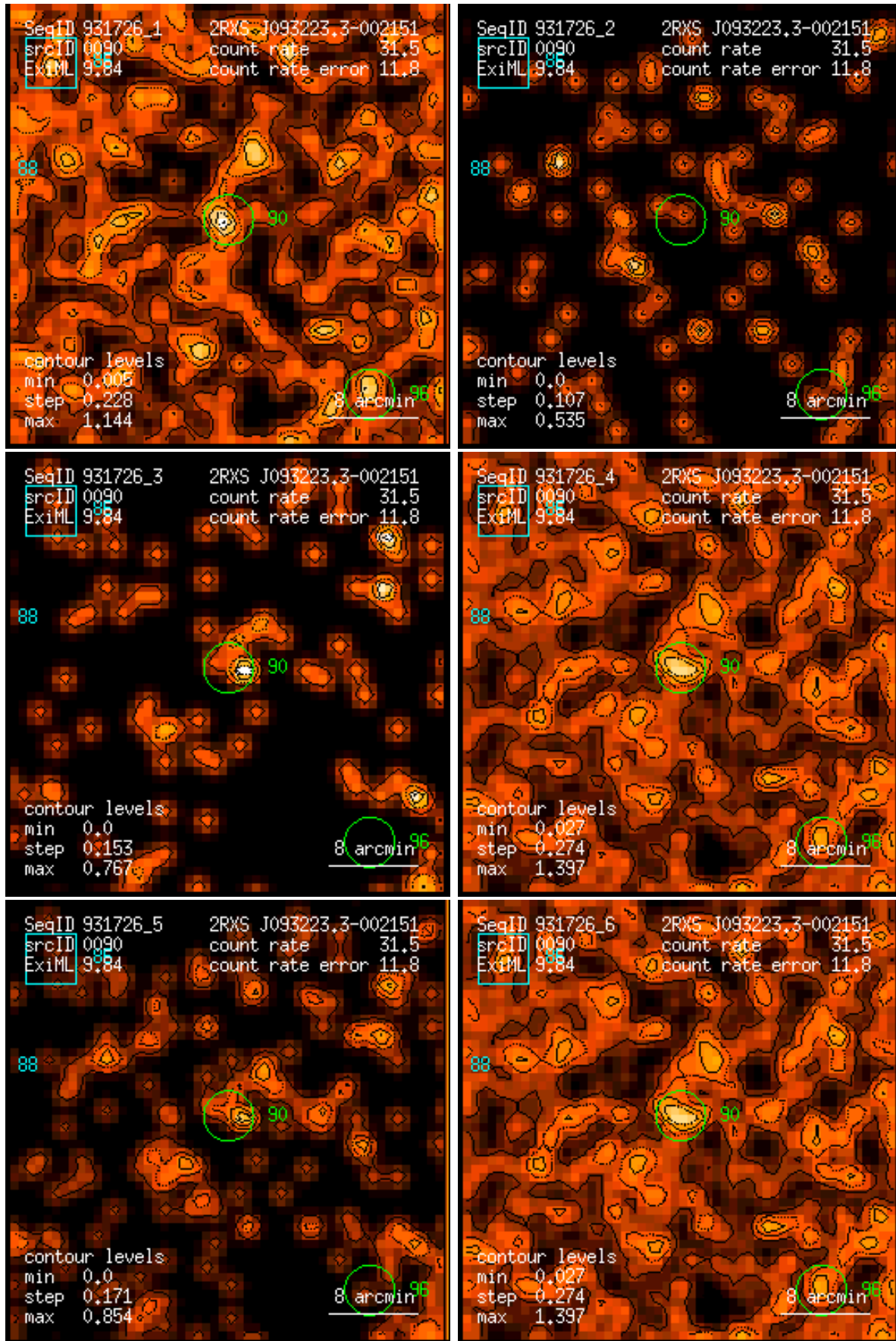
Figure 90: RASS 931726: detection 0090: band rate images, Gaussian filter: (1) PSPC channels 11 – 41, (2) 52 – 90, (3) 91 – 201, (4) 11 – 235, (5) 52 – 201, (6) 11 – 201. Broad band rates in counts/ks. Band rate contour levels in counts/ks/arcmin 2 .
