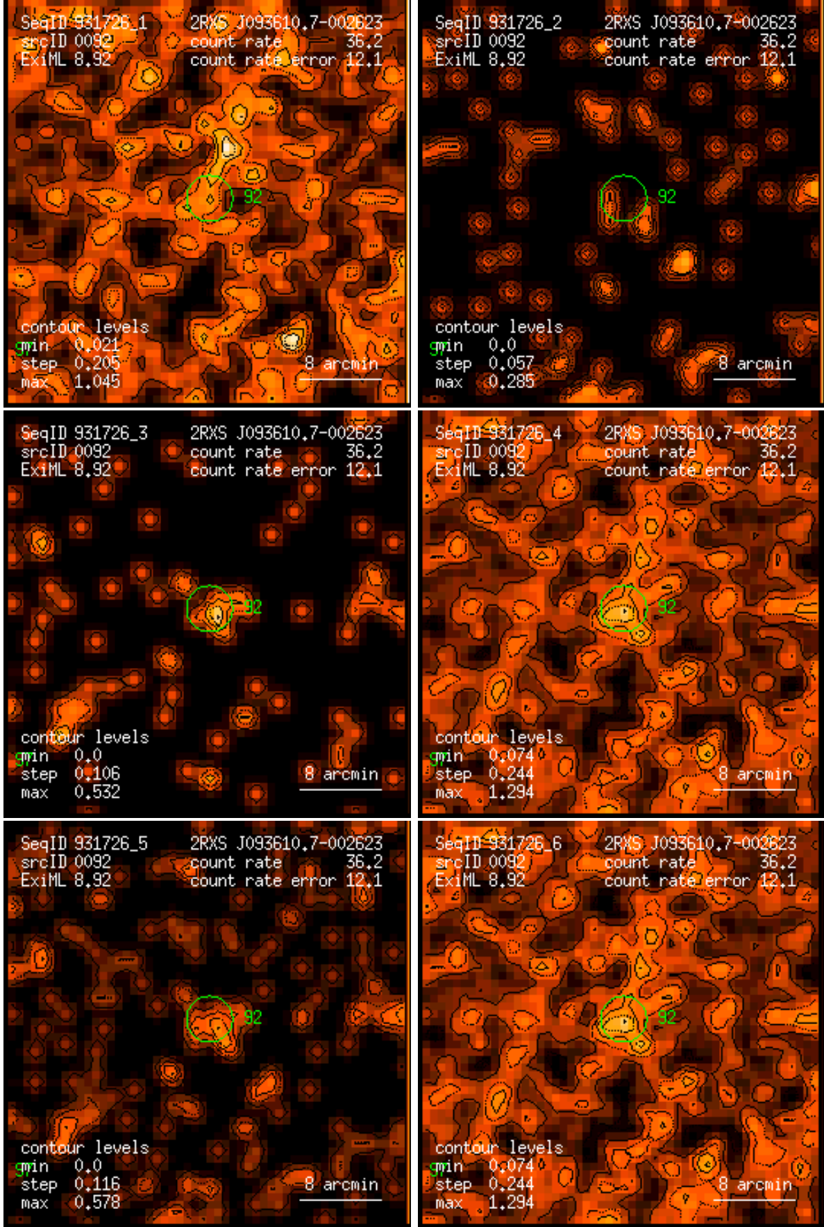
Figure 92: RASS 931726: detection 0092: band rate images, Gaussian filter: (1) PSPC channels 11 – 41, (2) 52 – 90, (3) 91 – 201, (4) 11 – 235, (5) 52 – 201, (6) 11 – 201. Broad band rates in counts/ks. Band rate contour levels in counts/ks/arcmin 2 .
