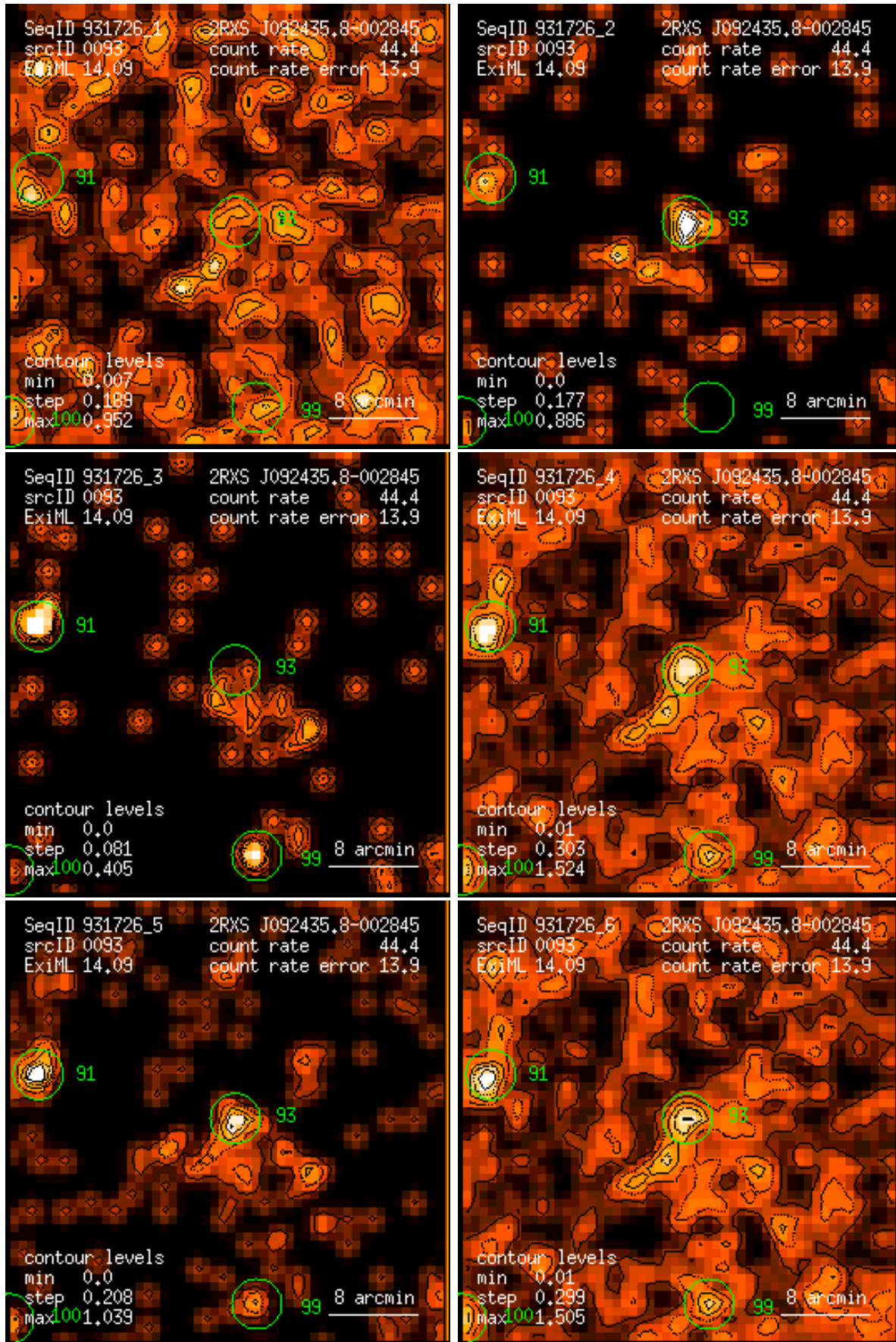
Figure 93: RASS 931726: detection 0093: band rate images, Gaussian filter: (1) PSPC channels 11 – 41, (2) 52 – 90, (3) 91 – 201, (4) 11 – 235, (5) 52 – 201, (6) 11 – 201. Broad band rates in counts/ks. Band rate contour levels in counts/ks/arcmin 2 .
