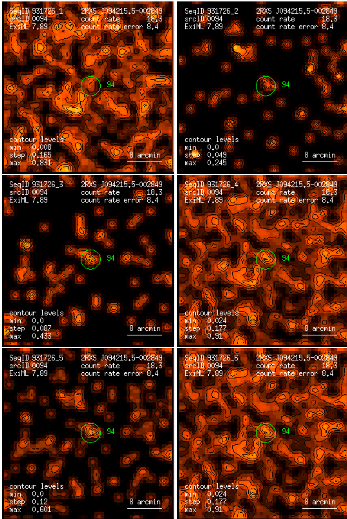
Figure 94: RASS 931726: detection 0094: band rate images, Gaussian filter: (1) PSPC channels 11 – 41, (2) 52 – 90, (3) 91 – 201, (4) 11 – 235, (5) 52 – 201, (6) 11 – 201. Broad band rates in counts/ks. Band rate contour levels in counts/ks/arcmin 2 .
