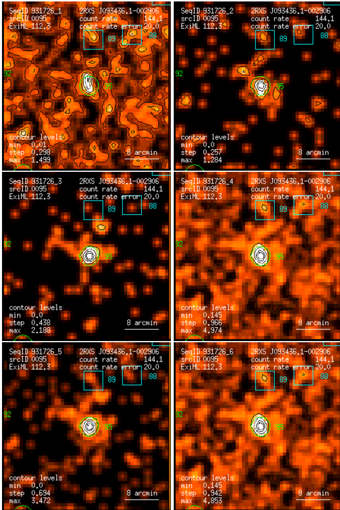
Figure 95: RASS 931726: detection 0095: band rate images, Gaussian filter: (1) PSPC channels 11 – 41, (2) 52 – 90, (3) 91 – 201, (4) 11 – 235, (5) 52 – 201, (6) 11 – 201. Broad band rates in counts/ks. Band rate contour levels in counts/ks/arcmin 2 .
