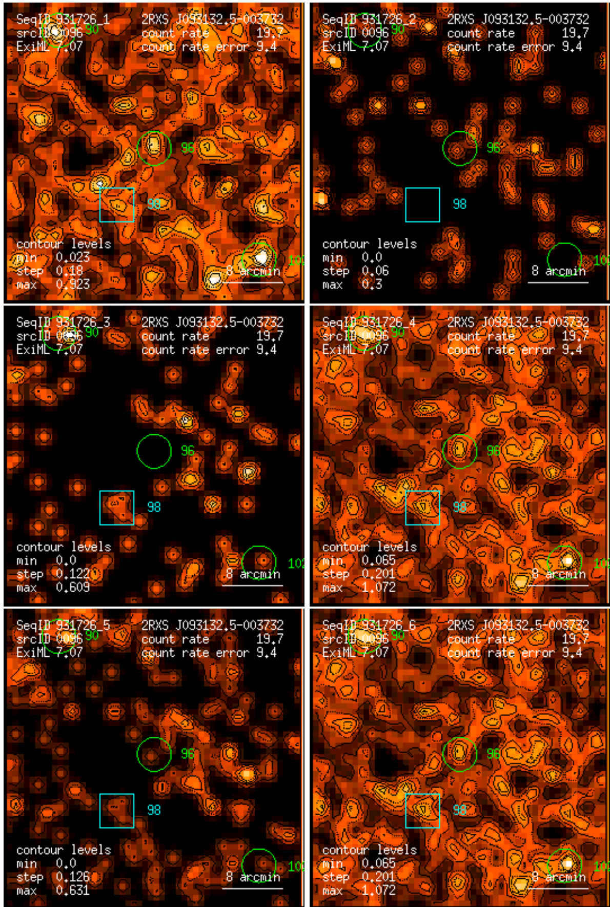
Figure 96: RASS 931726: detection 0096: band rate images, Gaussian filter: (1) PSPC channels 11 – 41, (2) 52 – 90, (3) 91 – 201, (4) 11 – 235, (5) 52 – 201, (6) 11 – 201. Broad band rates in counts/ks. Band rate contour levels in counts/ks/arcmin 2 .
