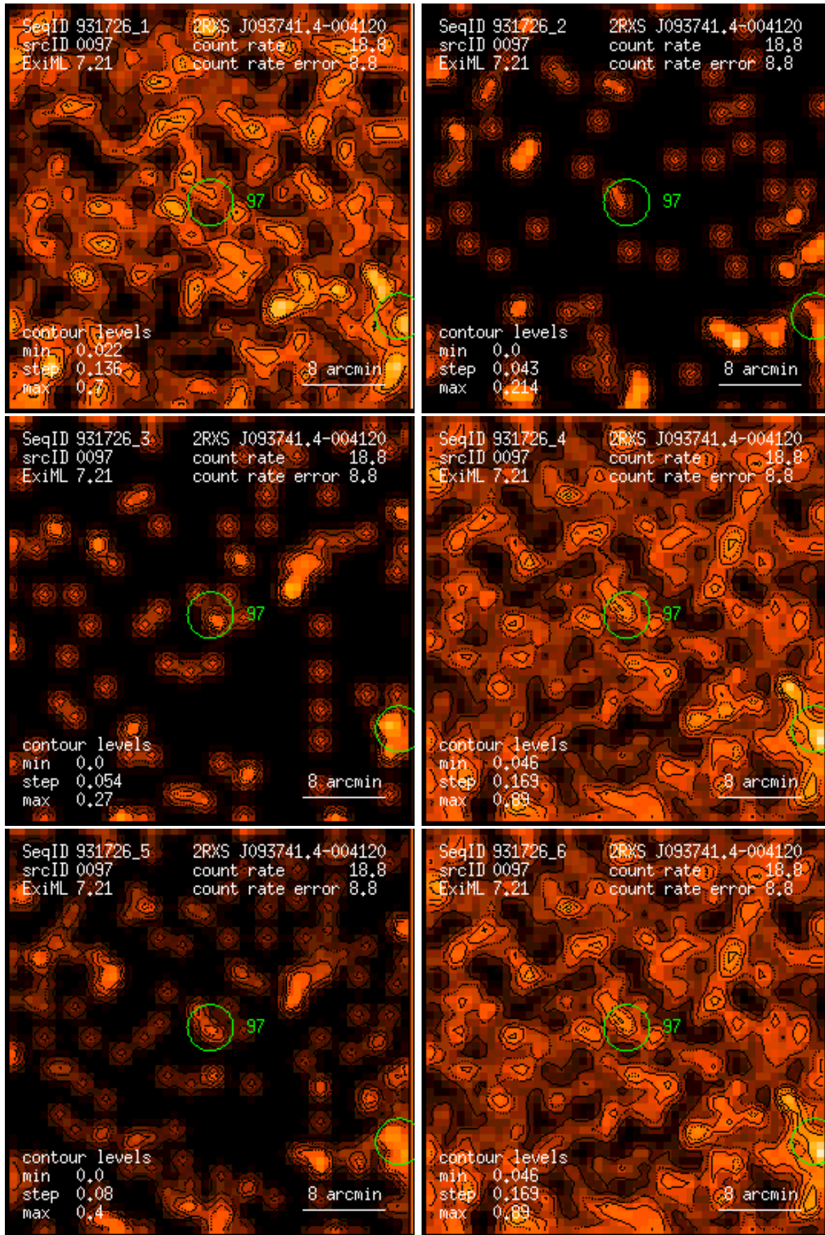
Figure 97: RASS 931726: detection 0097: band rate images, Gaussian filter: (1) PSPC channels 11 – 41, (2) 52 – 90, (3) 91 – 201, (4) 11 – 235, (5) 52 – 201, (6) 11 – 201. Broad band rates in counts/ks. Band rate contour levels in counts/ks/arcmin 2 .
