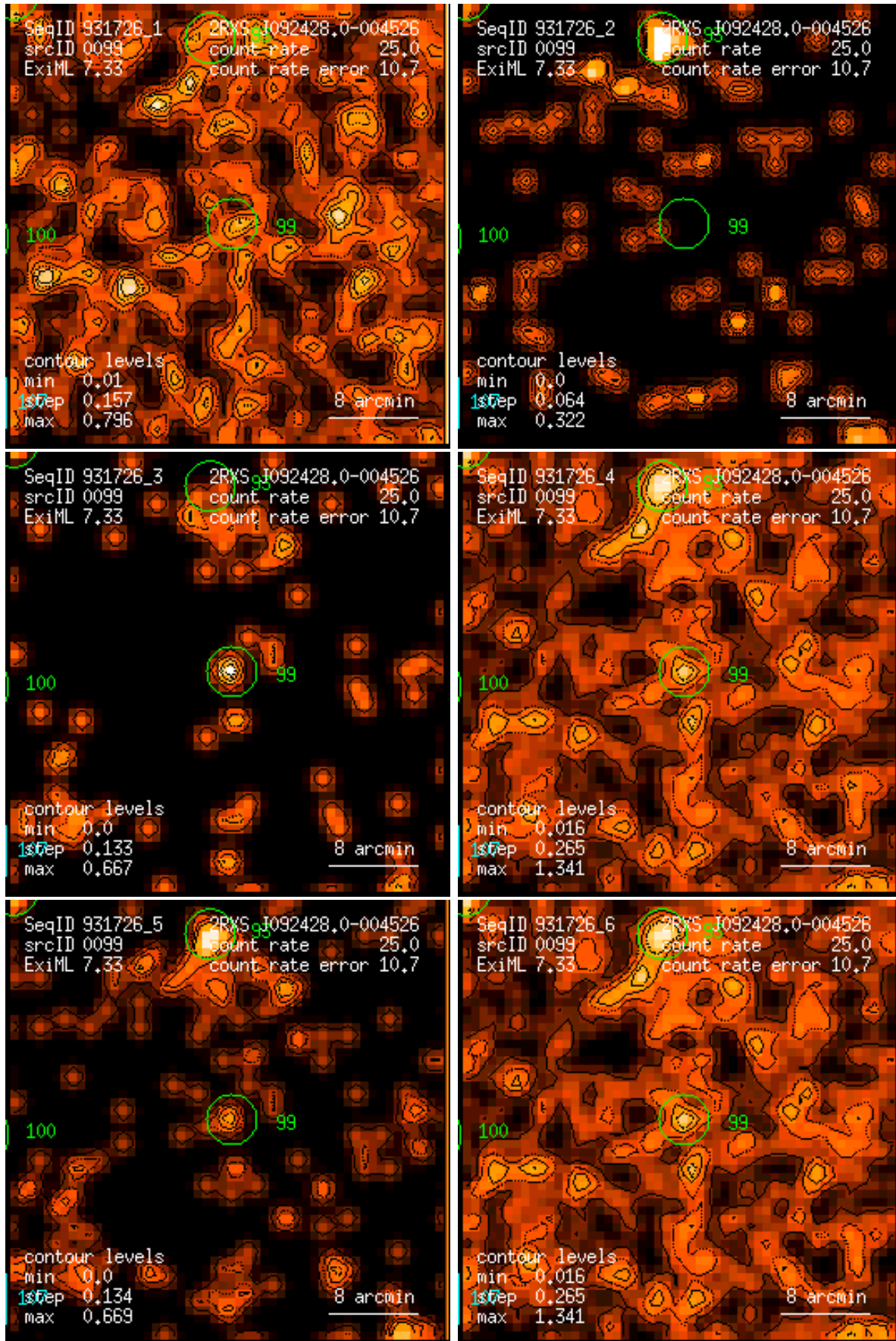
Figure 99: RASS 931726: detection 0099: band rate images, Gaussian filter: (1) PSPC channels 11 – 41, (2) 52 – 90, (3) 91 – 201, (4) 11 – 235, (5) 52 – 201, (6) 11 – 201. Broad band rates in counts/ks. Band rate contour levels in counts/ks/arcmin 2 .
