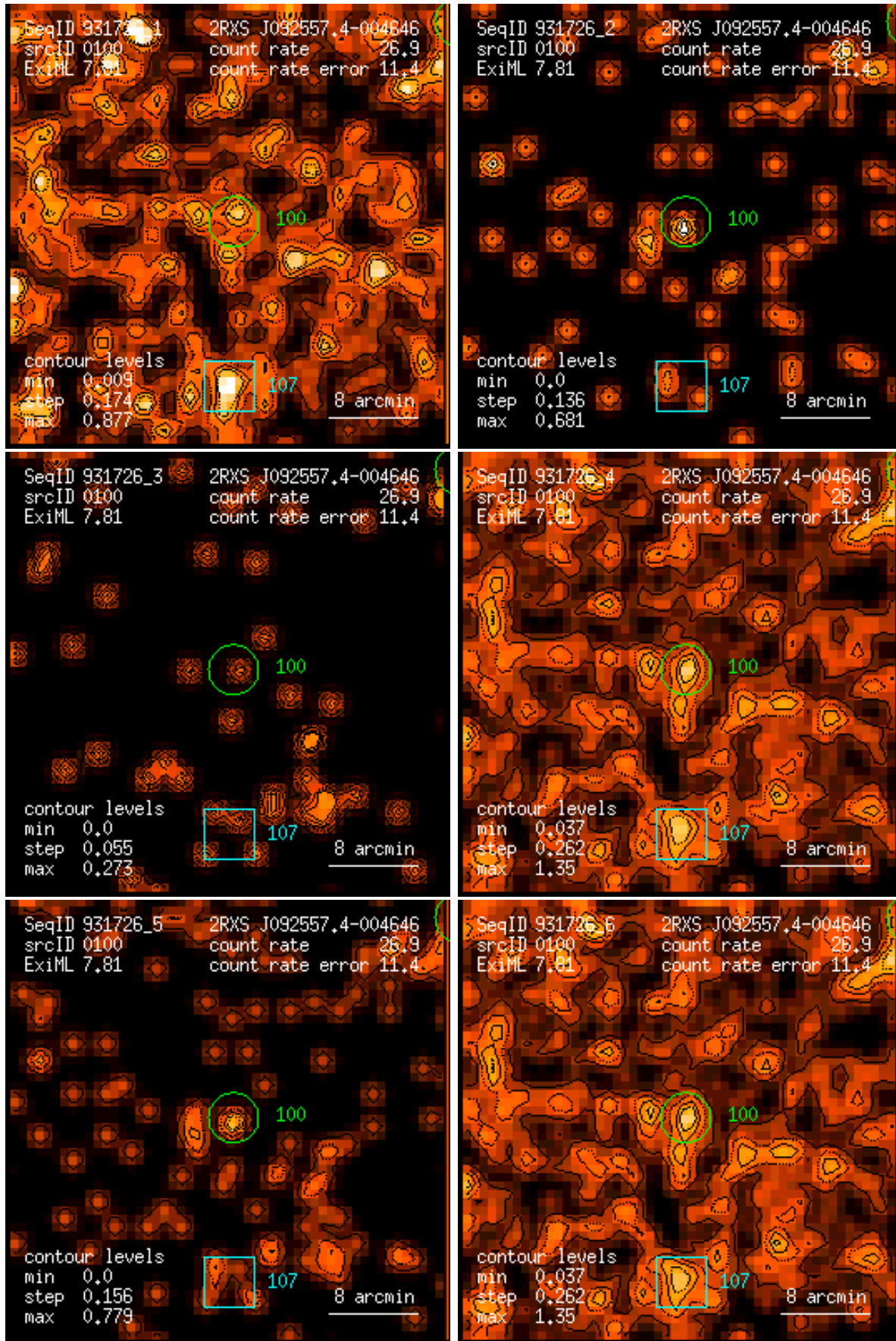
Figure 100: RASS 931726: detection 0100: band rate images, Gaussian filter: (1) PSPC channels 11 – 41, (2) 52 – 90, (3) 91 – 201, (4) 11 – 235, (5) 52 – 201, (6) 11 – 201. Broad band rates in counts/ks. Band rate contour levels in counts/ks/arcmin 2 .
