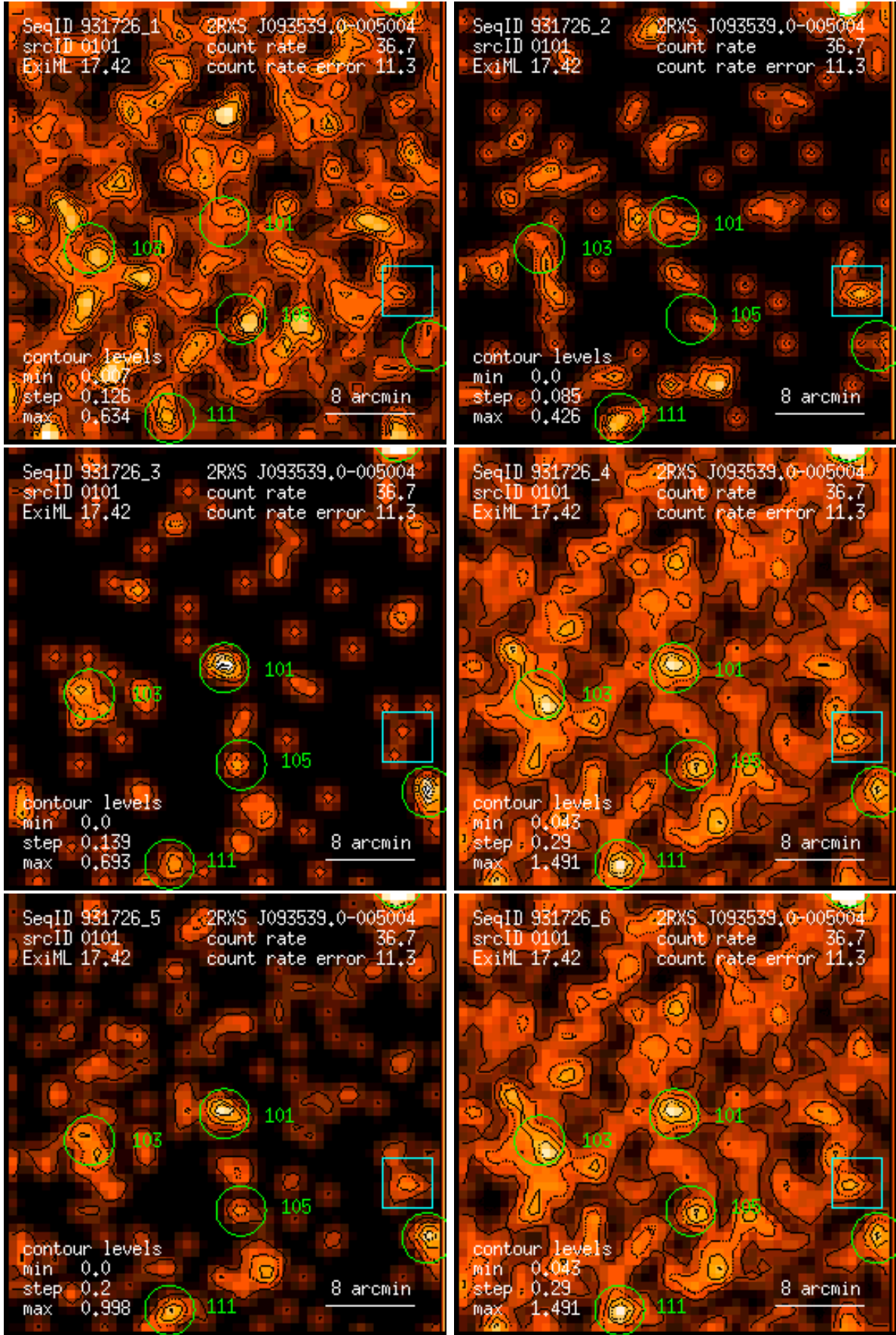
Figure 101: RASS 931726: detection 0101: band rate images, Gaussian filter: (1) PSPC channels 11 – 41, (2) 52 – 90, (3) 91 – 201, (4) 11 – 235, (5) 52 – 201, (6) 11 – 201. Broad band rates in counts/ks. Band rate contour levels in counts/ks/arcmin 2 .
