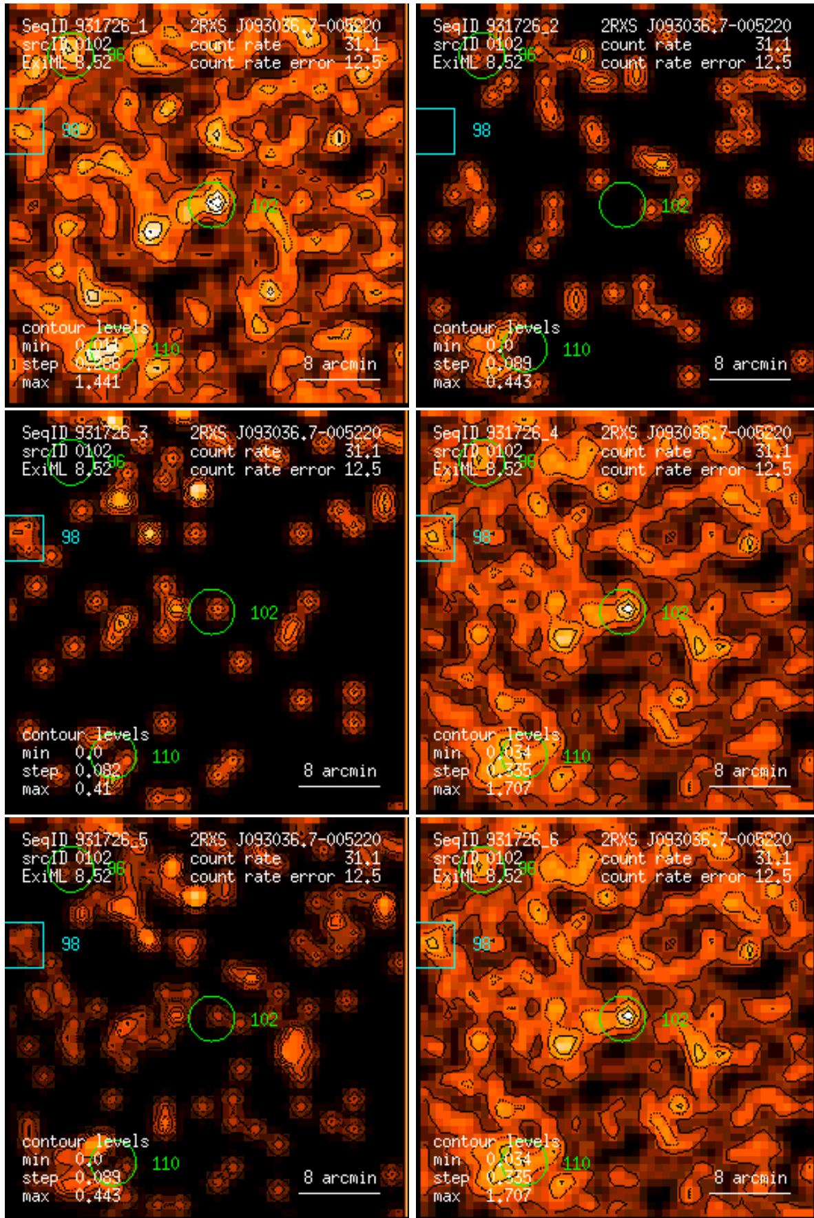
Figure 102: RASS 931726: detection 0102: band rate images, Gaussian filter: (1) PSPC channels 11 – 41, (2) 52 – 90, (3) 91 – 201, (4) 11 – 235, (5) 52 – 201, (6) 11 – 201. Broad band rates in counts/ks. Band rate contour levels in counts/ks/arcmin 2 .
