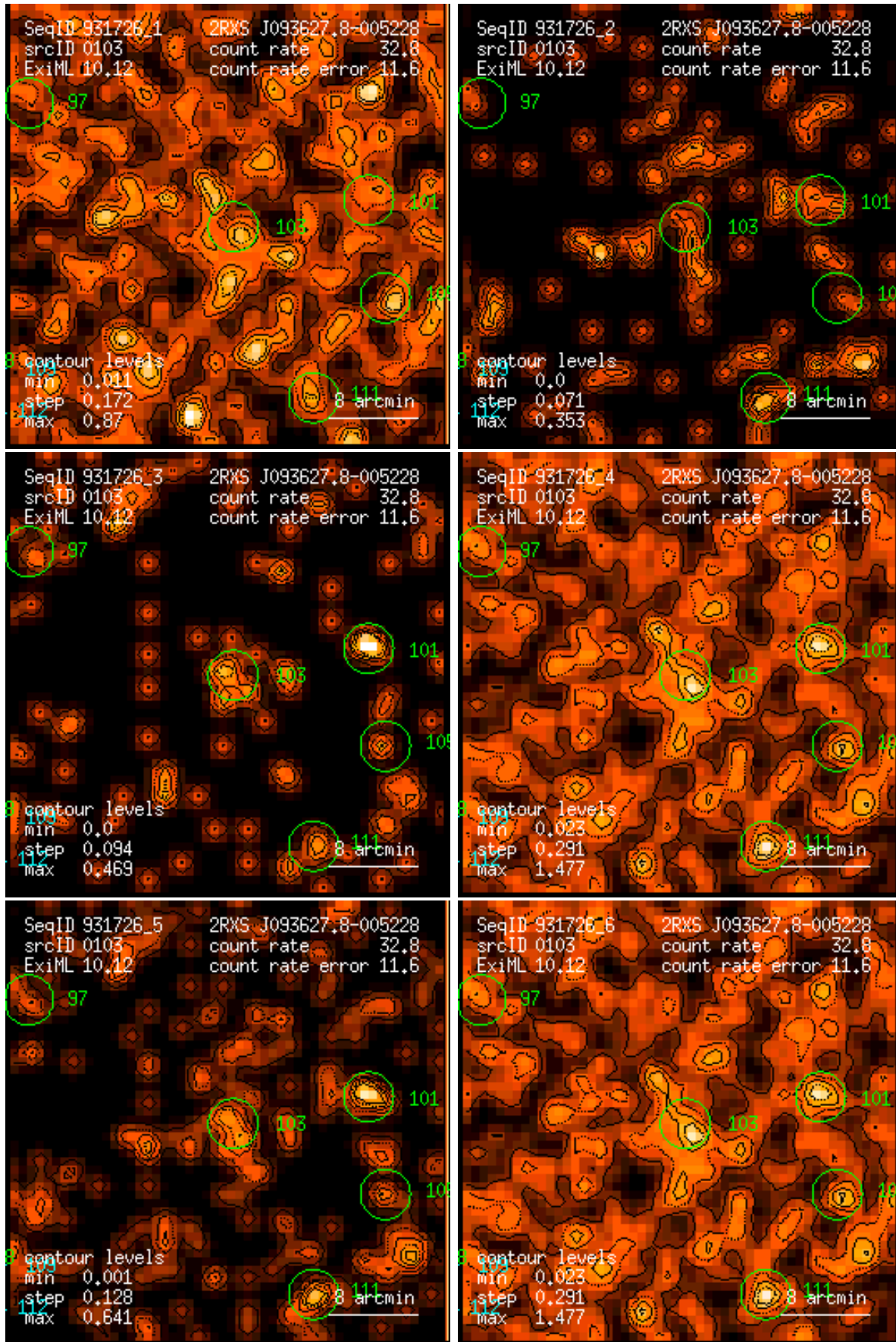
Figure 103: RASS 931726: detection 0103: band rate images, Gaussian filter: (1) PSPPC channels 11 – 41, (2) 52 – 90, (3) 91 – 201, (4) 11 – 235, (5) 52 – 201, (6) 11 – 201. Broad band rates in counts/ks. Band rate contour levels in counts/ks/arcmin 2 .
