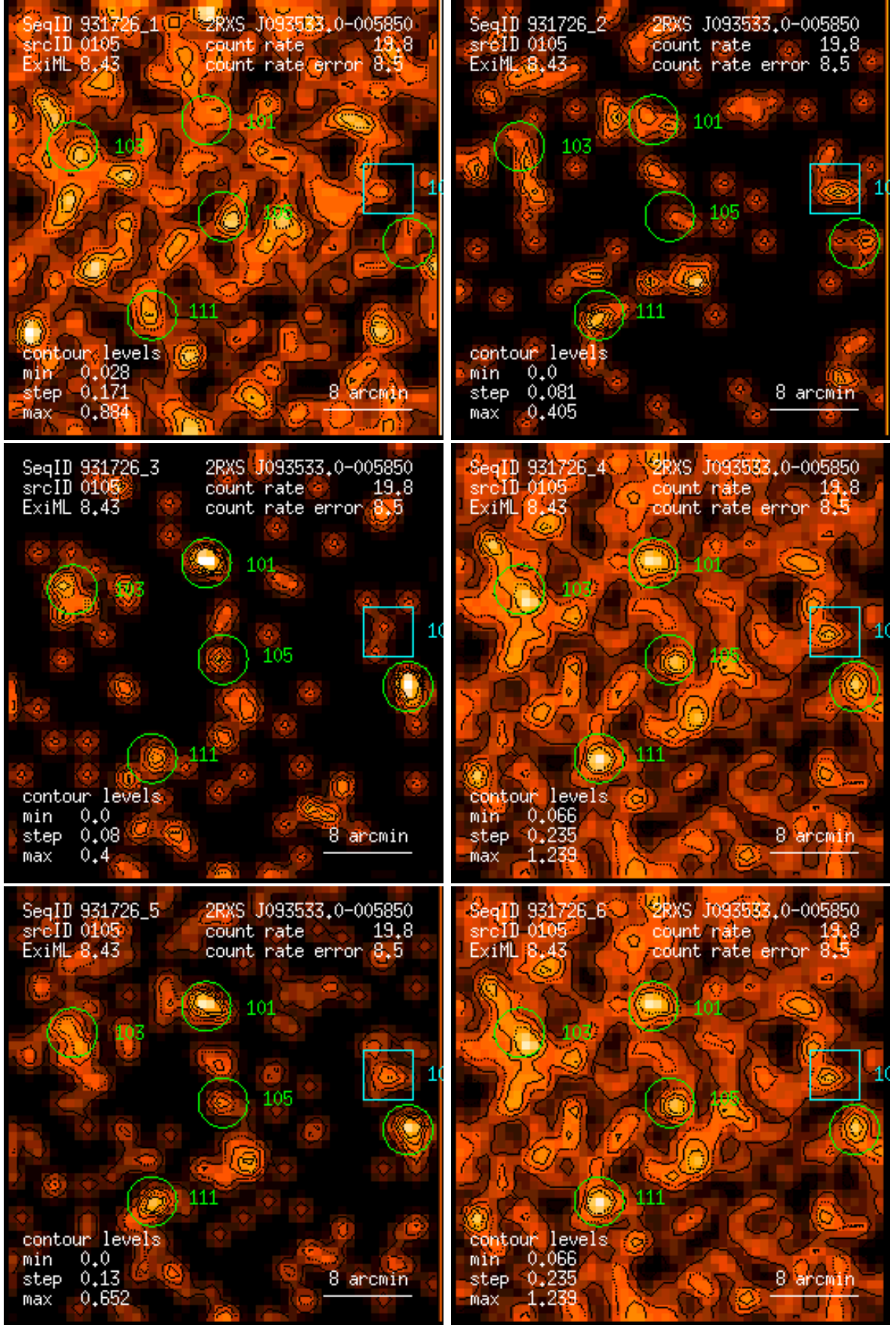
Figure 105: RASS 931726: detection 0105: band rate images, Gaussian filter: (1) PSPC channels 11 – 41, (2) 52 – 90, (3) 91 – 201, (4) 11 – 235, (5) 52 – 201, (6) 11 – 201. Broad band rates in counts/ks. Band rate contour levels in counts/ks/arcmin 2 .
