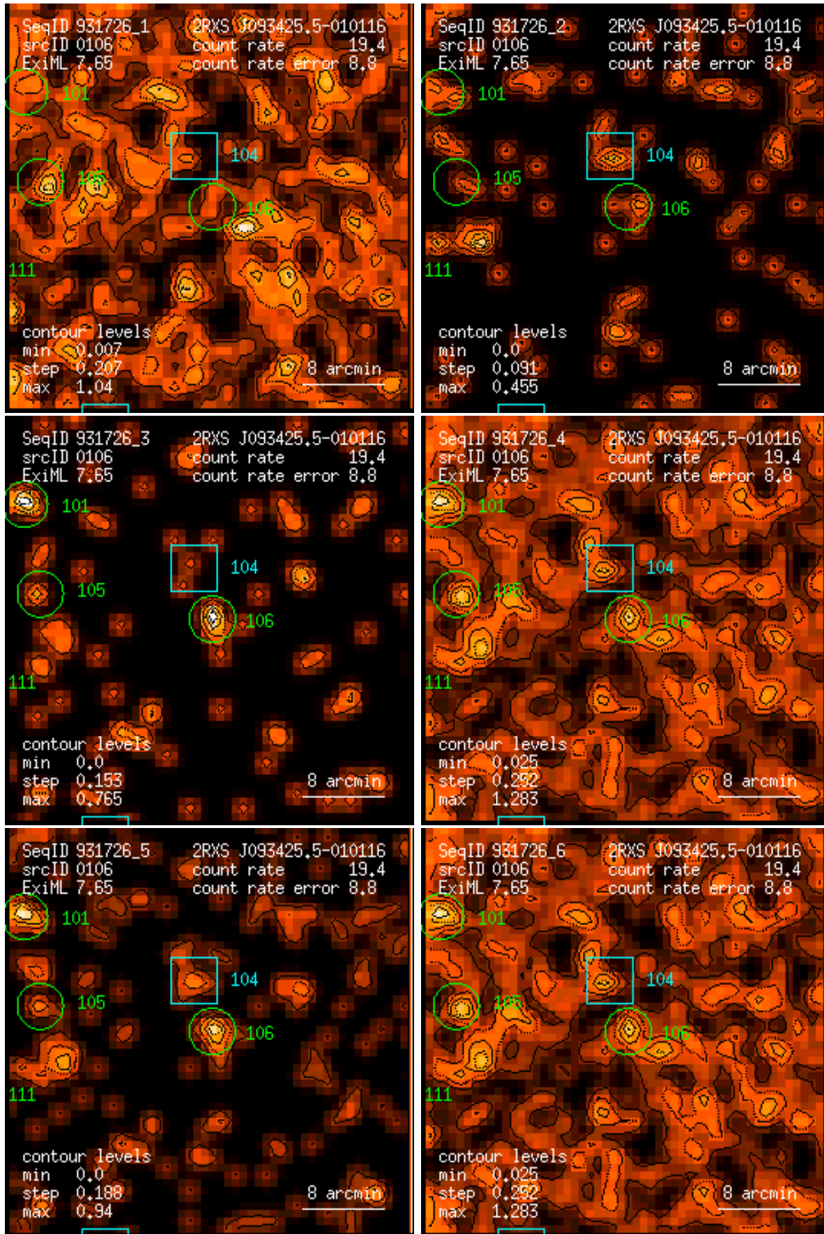
Figure 106: RASS 931726: detection 0106: band rate images, Gaussian filter: (1) PSPC channels 11 – 41, (2) 52 – 90, (3) 91 – 201, (4) 11 – 235, (5) 52 – 201, (6) 11 – 201. Broad band rates in counts/ks. Band rate contour levels in counts/ks/arcmin 2 .
