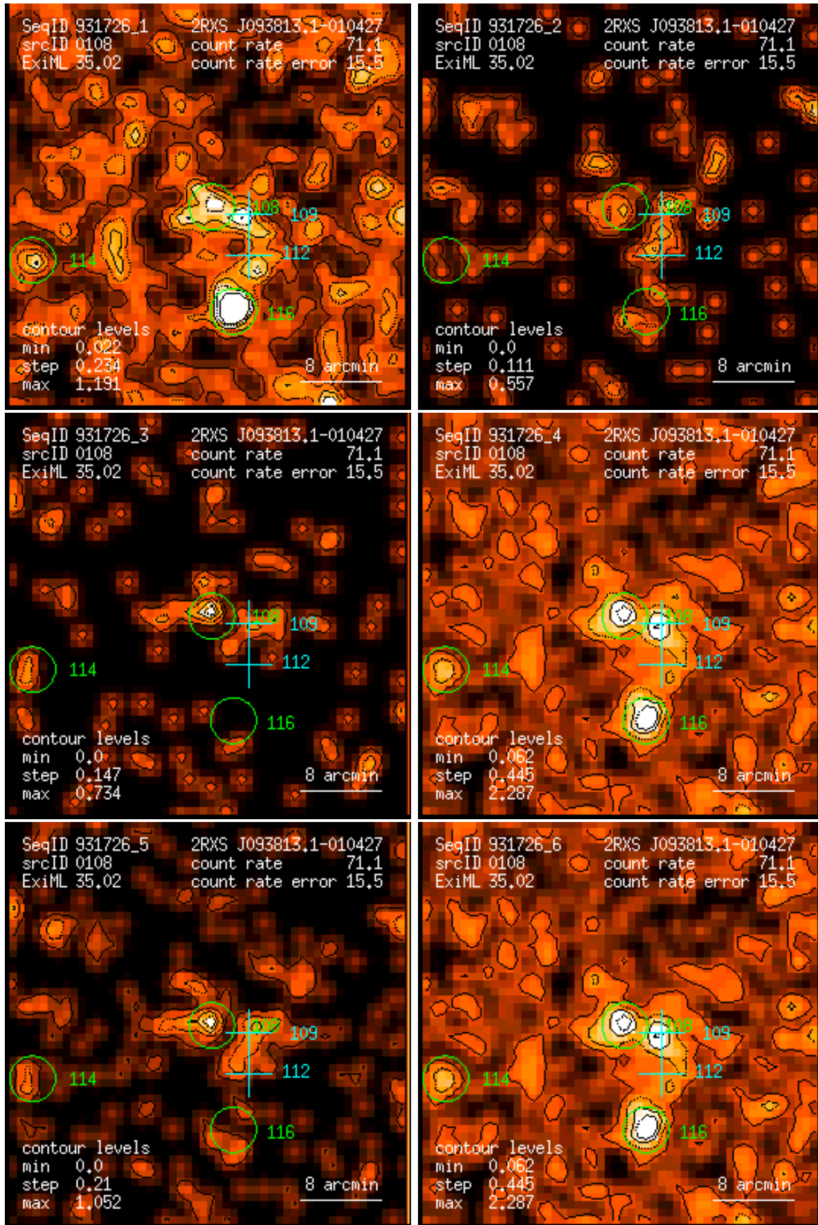
Figure 108: RASS 931726: detection 0108: band rate images, Gaussian filter: (1) PSPC channels 11 – 41, (2) 52 – 90, (3) 91 – 201, (4) 11 – 235, (5) 52 – 201, (6) 11 – 201. Broad band rates in counts/ks. Band rate contour levels in counts/ks/arcmin 2 .
