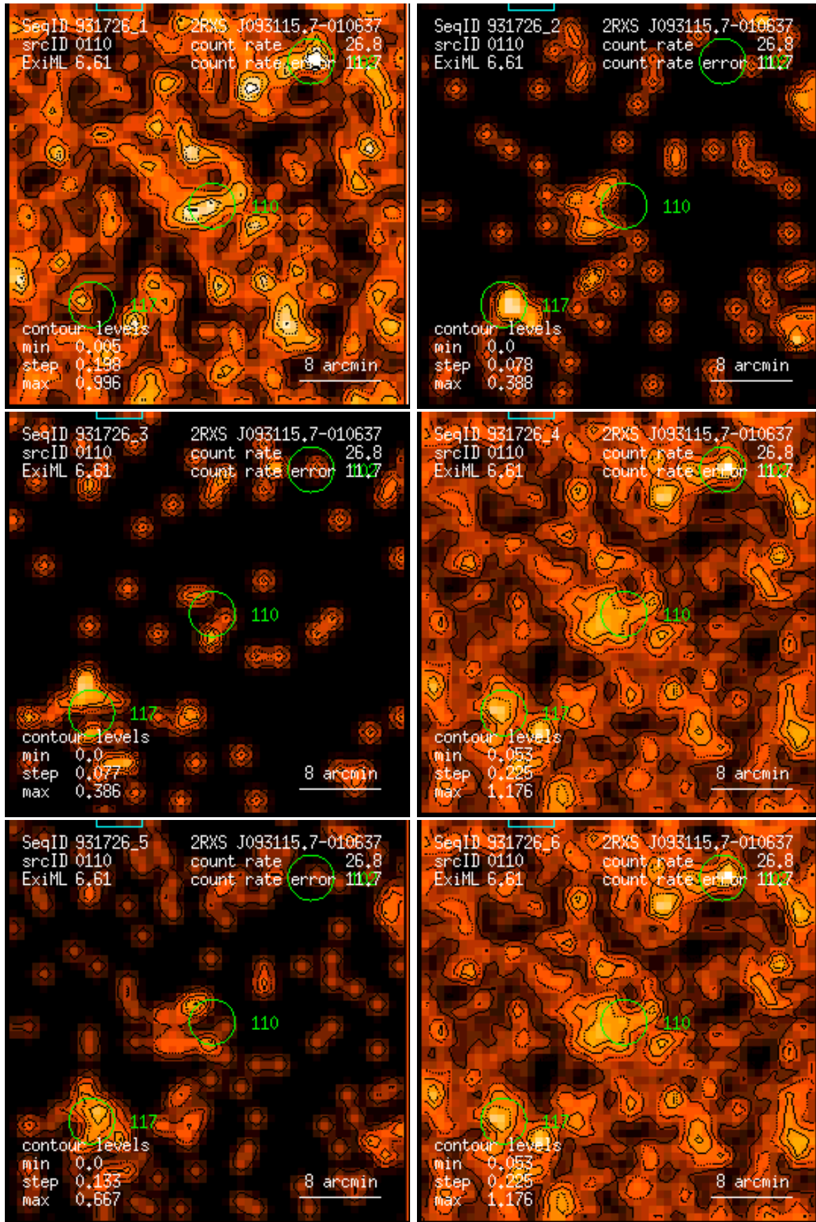
Figure 110: RASS 931726: detection 0110: band rate images, Gaussian filter: (1) PSPC channels 11 – 41, (2) 52 – 90, (3) 91 – 201, (4) 11 – 235, (5) 52 – 201, (6) 11 – 201. Broad band rates in counts/ks. Band rate contour levels in counts/ks/arcmin 2 .
