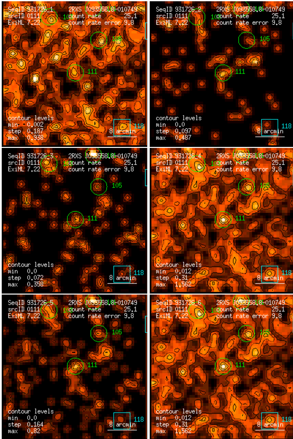
Figure 111: RASS 931726: detection 0111: band rate images, Gaussian filter: (1) PSPC channels 11 – 41, (2) 52 – 90, (3) 91 – 201, (4) 11 – 235, (5) 52 – 201, (6) 11 – 201. Broad band rates in counts/ks. Band rate contour levels in counts/ks/arcmin 2 .
