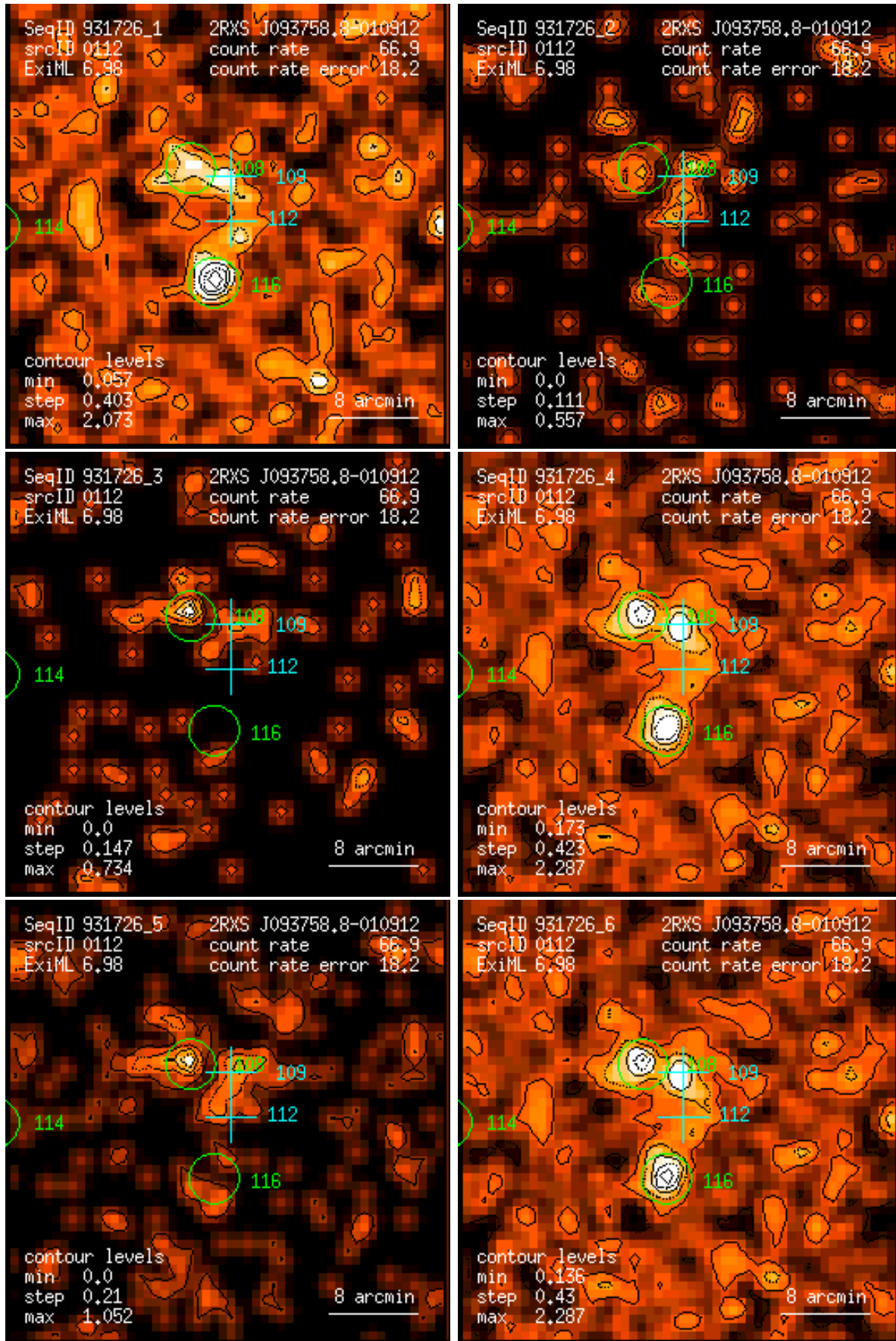
Figure 112: RASS 931726: detection 0112: band rate images, Gaussian filter: (1) PSPC channels 11 – 41, (2) 52 – 90, (3) 91 – 201, (4) 11 – 235, (5) 52 – 201, (6) 11 – 201. Broad band rates in counts/ks. Band rate contour levels in counts/ks/arcmin 2 .
