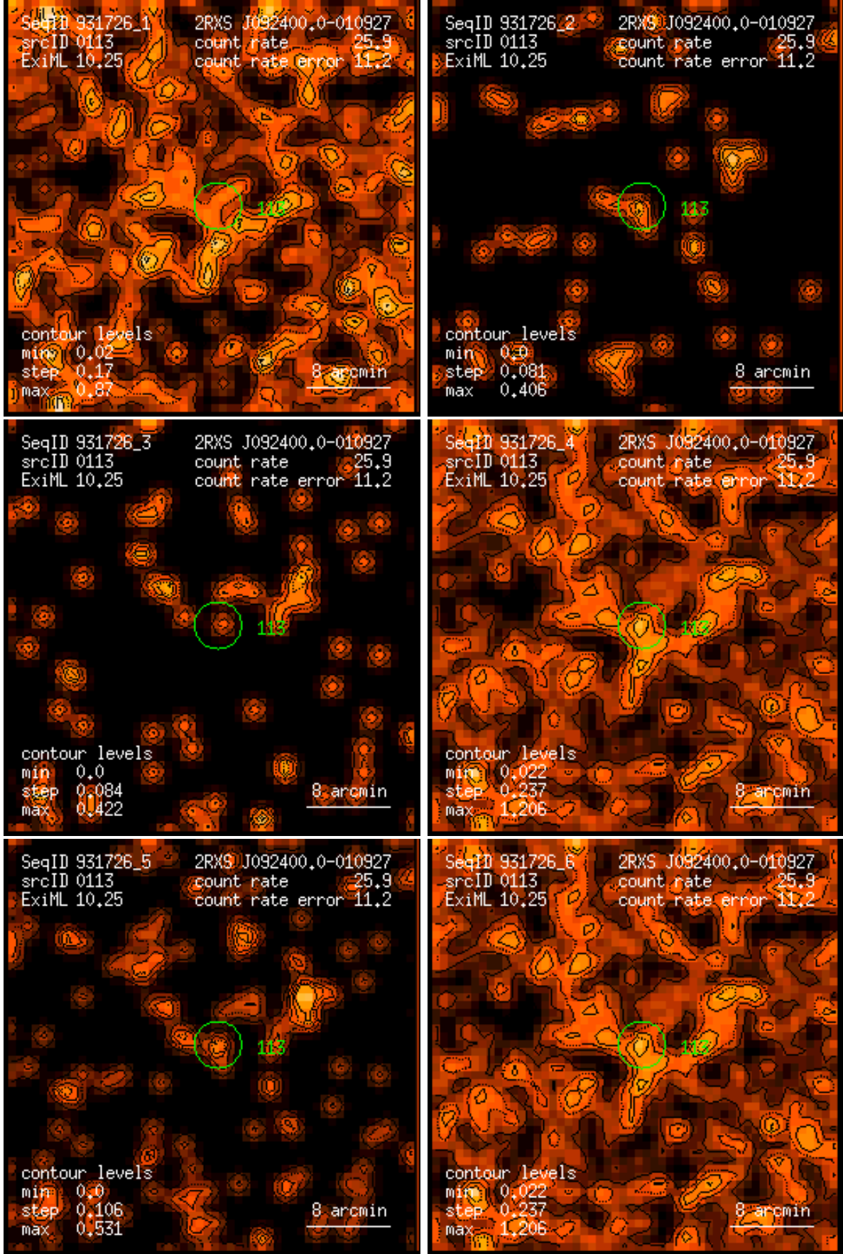
Figure 113: RASS 931726: detection 0113: band rate images, Gaussian filter: (1) PSPC channels 11 – 41, (2) 52 – 90, (3) 91 – 201, (4) 11 – 235, (5) 52 – 201, (6) 11 – 201. Broad band rates in counts/ks. Band rate contour levels in counts/ks/arcmin 2 .
