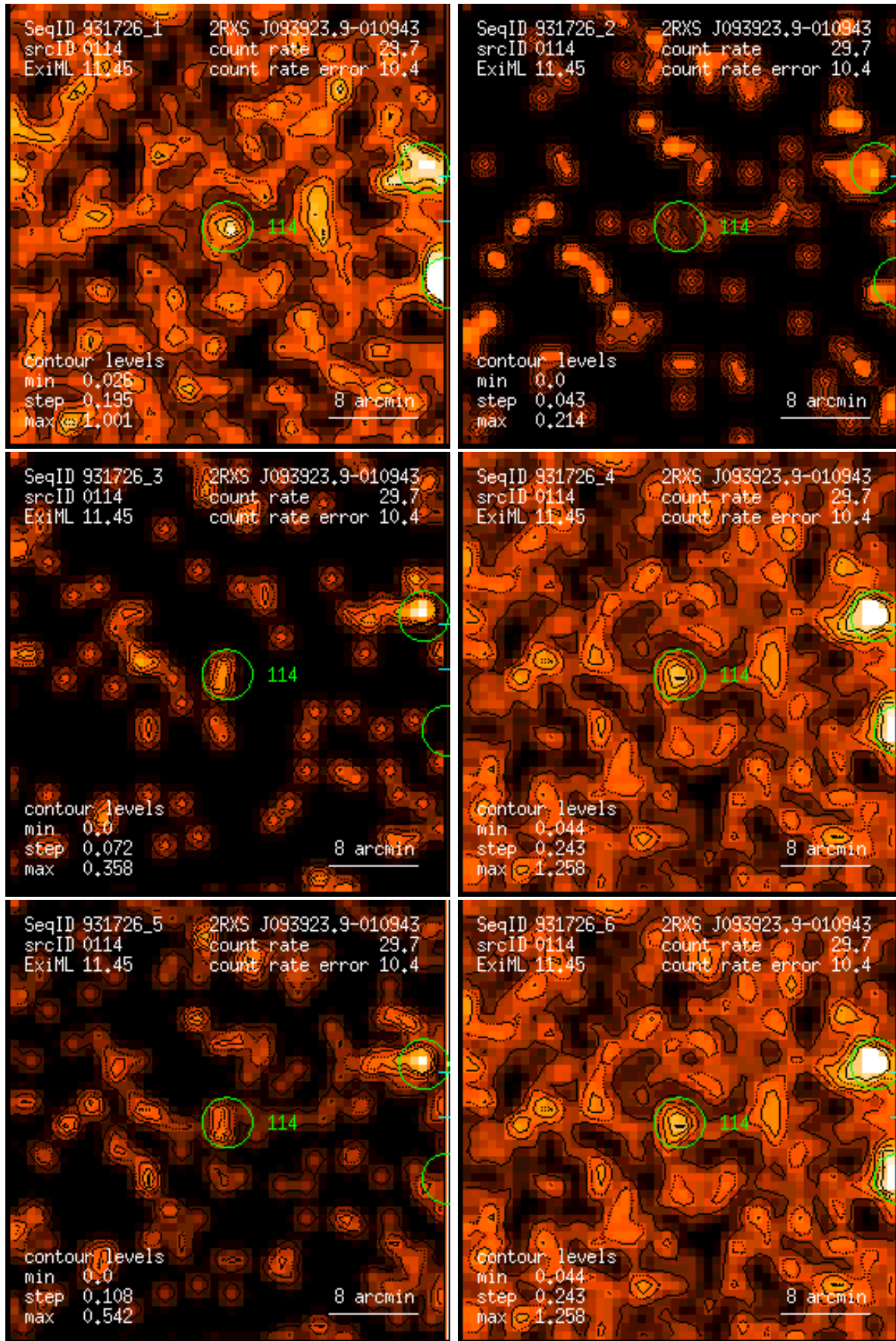
Figure 114: RASS 931726: detection 0114: band rate images, Gaussian filter: (1) PSPC channels 11 – 41, (2) 52 – 90, (3) 91 – 201, (4) 11 – 235, (5) 52 – 201, (6) 11 – 201. Broad band rates in counts/ks. Band rate contour levels in counts/ks/arcmin 2 .
