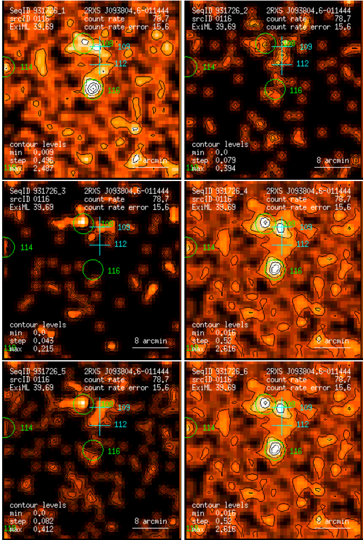
Figure 116: RASS 931726: detection 0116: band rate images, Gaussian filter: (1) PSPC channels 11 – 41, (2) 52 – 90, (3) 91 – 201, (4) 11 – 235, (5) 52 – 201, (6) 11 – 201. Broad band rates in counts/ks. Band rate contour levels in counts/ks/arcmin 2 .
