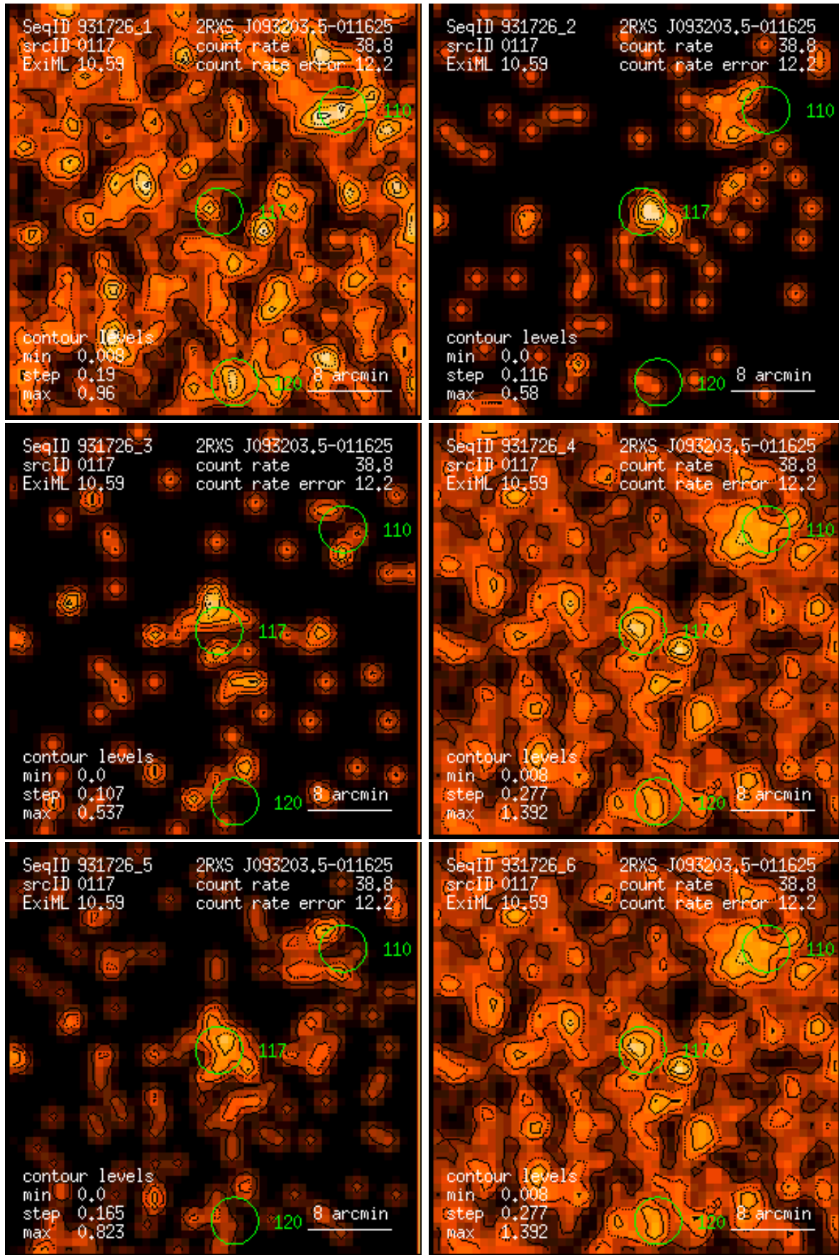
Figure 117: RASS 931726: detection 0117: band rate images, Gaussian filter: (1) PSPC channels 11 – 41, (2) 52 – 90, (3) 91 – 201, (4) 11 – 235, (5) 52 – 201, (6) 11 – 201. Broad band rates in counts/ks. Band rate contour levels in counts/ks/arcmin 2 .
