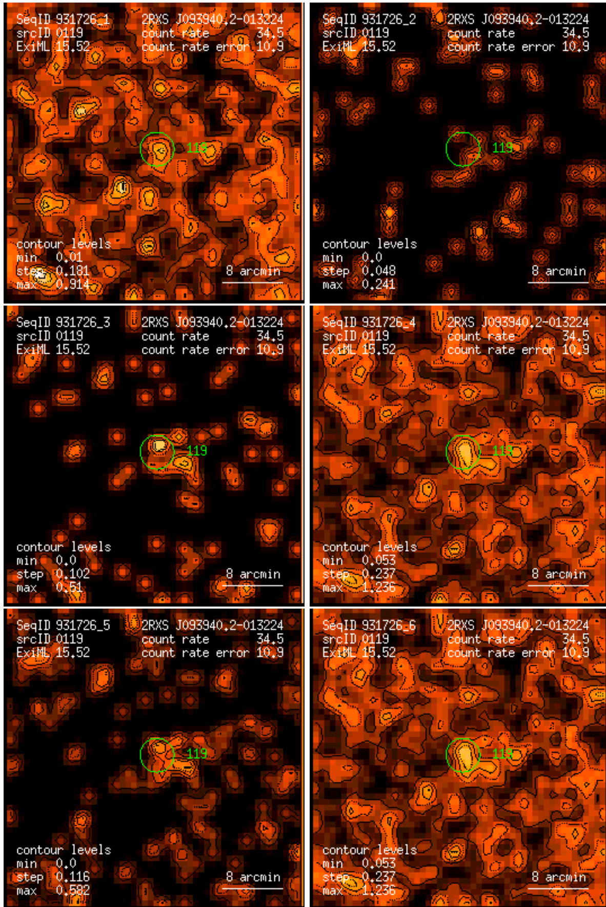
Figure 119: RASS 931726: detection 0119: band rate images, Gaussian filter: (1) PSPC channels 11 – 41, (2) 52 – 90, (3) 91 – 201, (4) 11 – 235, (5) 52 – 201, (6) 11 – 201. Broad band rates in counts/ks. Band rate contour levels in counts/ks/arcmin 2 .
