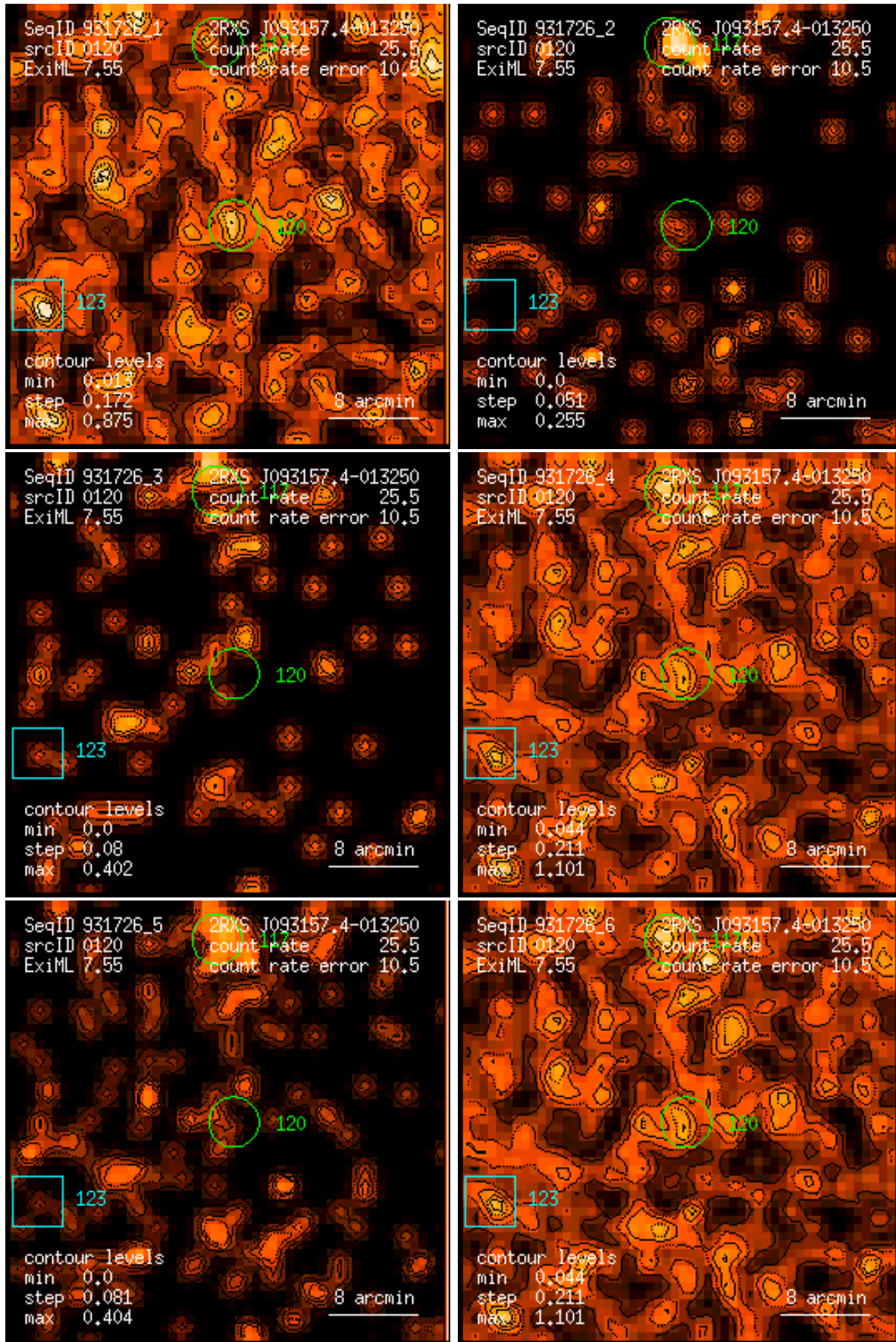
Figure 120: RASS 931726: detection 0120: band rate images, Gaussian filter: (1) PSPC channels 11 – 41, (2) 52 – 90, (3) 91 – 201, (4) 11 – 235, (5) 52 – 201, (6) 11 – 201. Broad band rates in counts/ks. Band rate contour levels in counts/ks/arcmin 2 .
