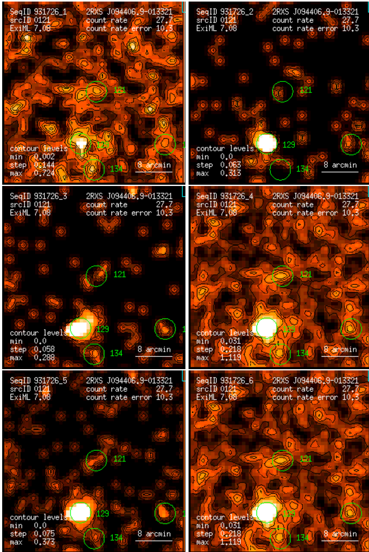
Figure 121: RASS 931726: detection 0121: band rate images, Gaussian filter: (1) PSPC channels 11 – 41, (2) 52 – 90, (3) 91 – 201, (4) 11 – 235, (5) 52 – 201, (6) 11 – 201. Broad band rates in counts/ks. Band rate contour levels in counts/ks/arcmin 2 .
