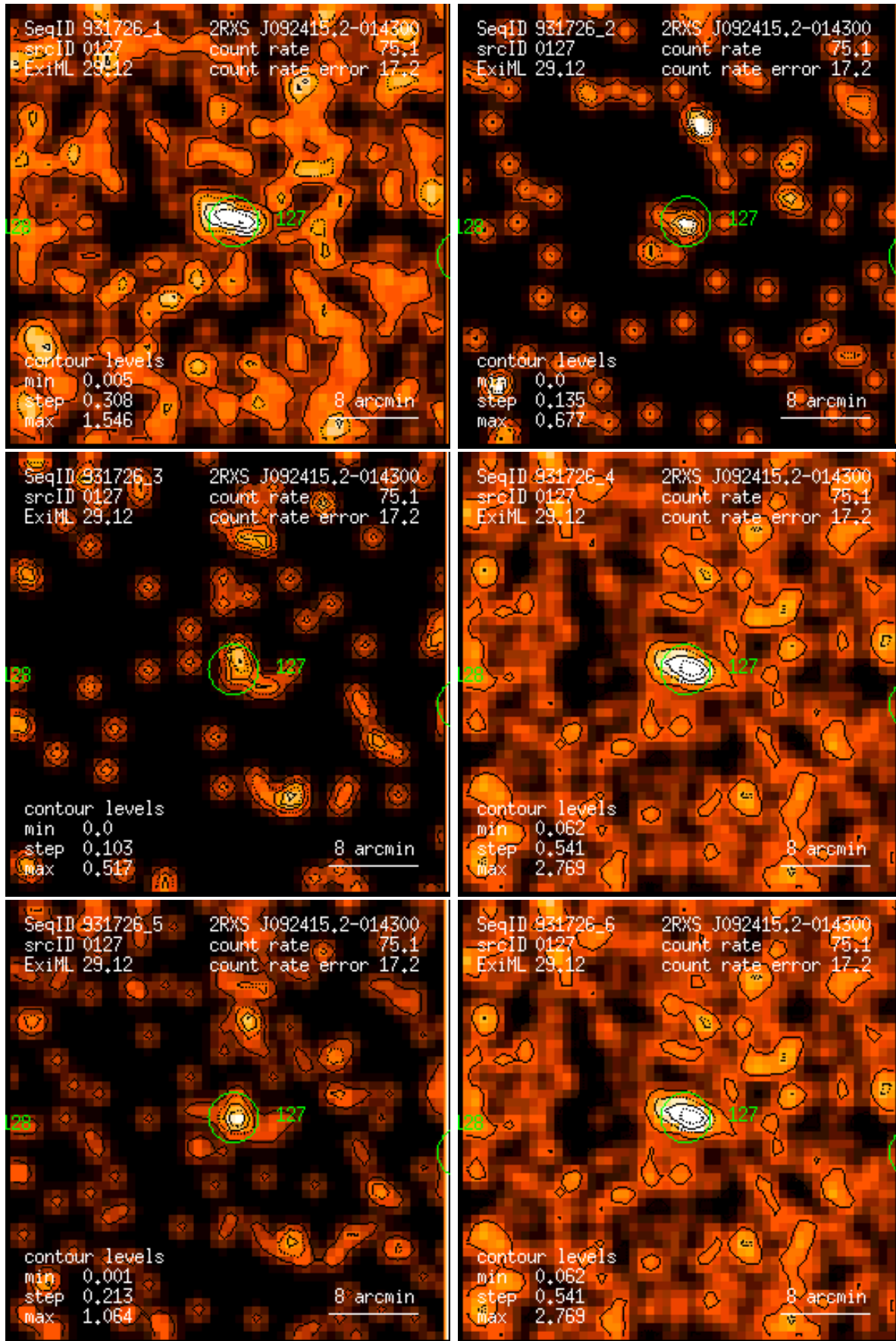
Figure 127: RASS 931726: detection 0127: band rate images, Gaussian filter: (1) PSPC channels 11 – 41, (2) 52 – 90, (3) 91 – 201, (4) 11 – 235, (5) 52 – 201, (6) 11 – 201. Broad band rates in counts/ks. Band rate contour levels in counts/ks/arcmin 2 .
