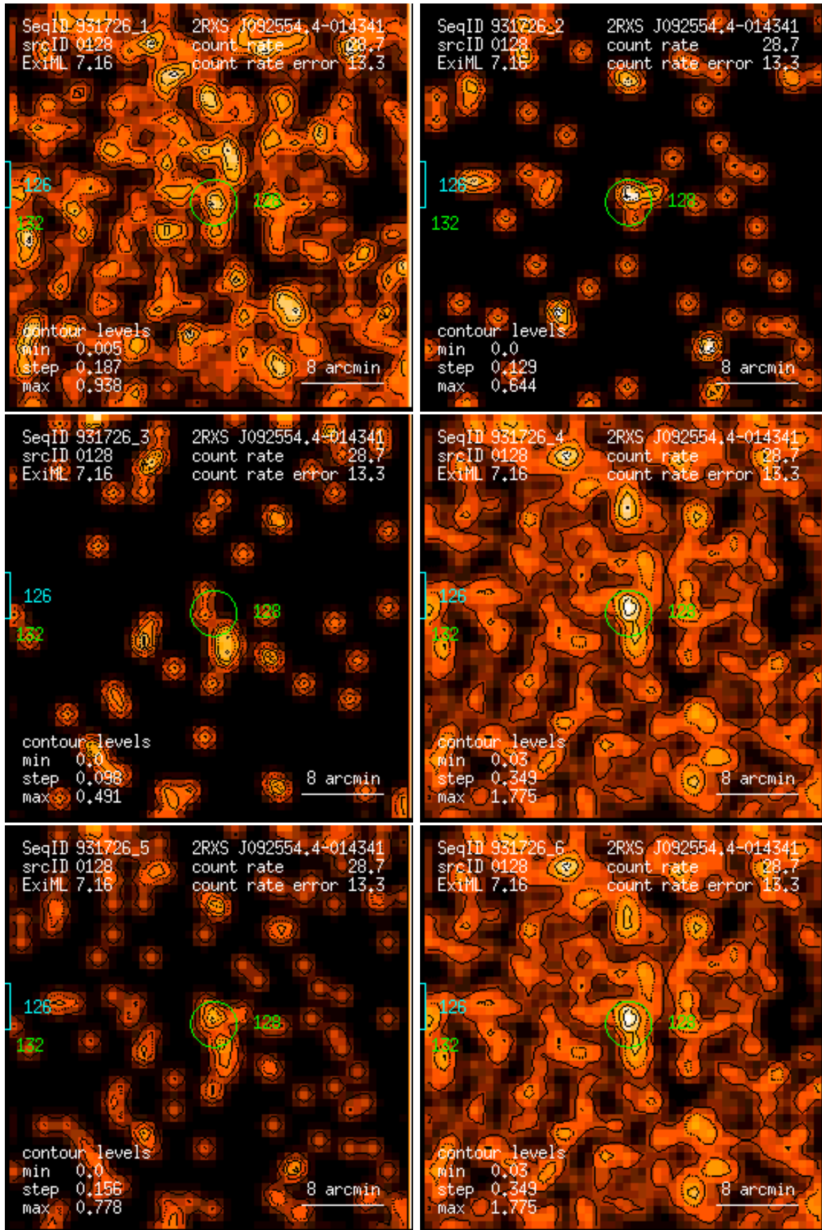
Figure 128: RASS 931726: detection 0128: band rate images, Gaussian filter: (1) PSPC channels 11 – 41, (2) 52 – 90, (3) 91 – 201, (4) 11 – 235, (5) 52 – 201, (6) 11 – 201. Broad band rates in counts/ks. Band rate contour levels in counts/ks/arcmin 2 .
