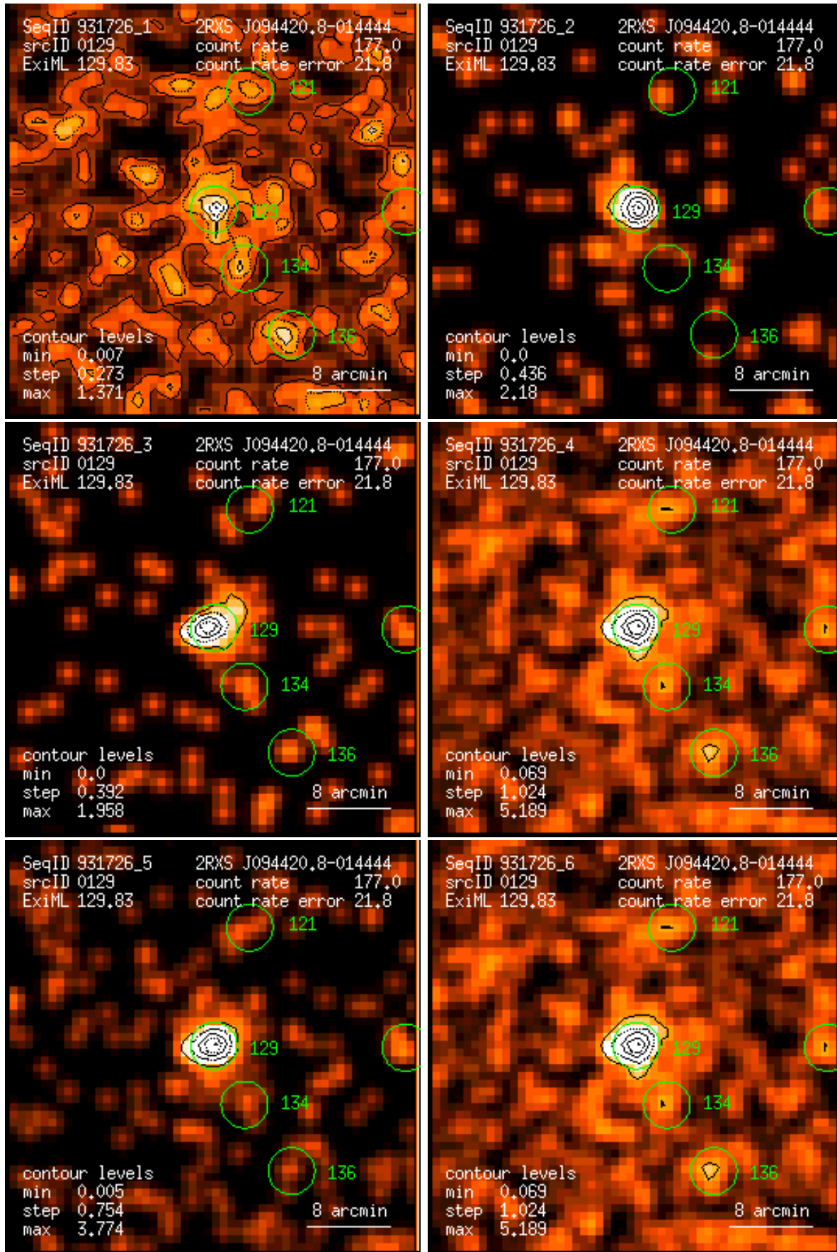
Figure 129: RASS 931726: detection 0129: band rate images, Gaussian filter: (1) PSPC channels 11 – 41, (2) 52 – 90, (3) 91 – 201, (4) 11 – 235, (5) 52 – 201, (6) 11 – 201. Broad band rates in counts/ks. Band rate contour levels in counts/ks/arcmin 2 .
