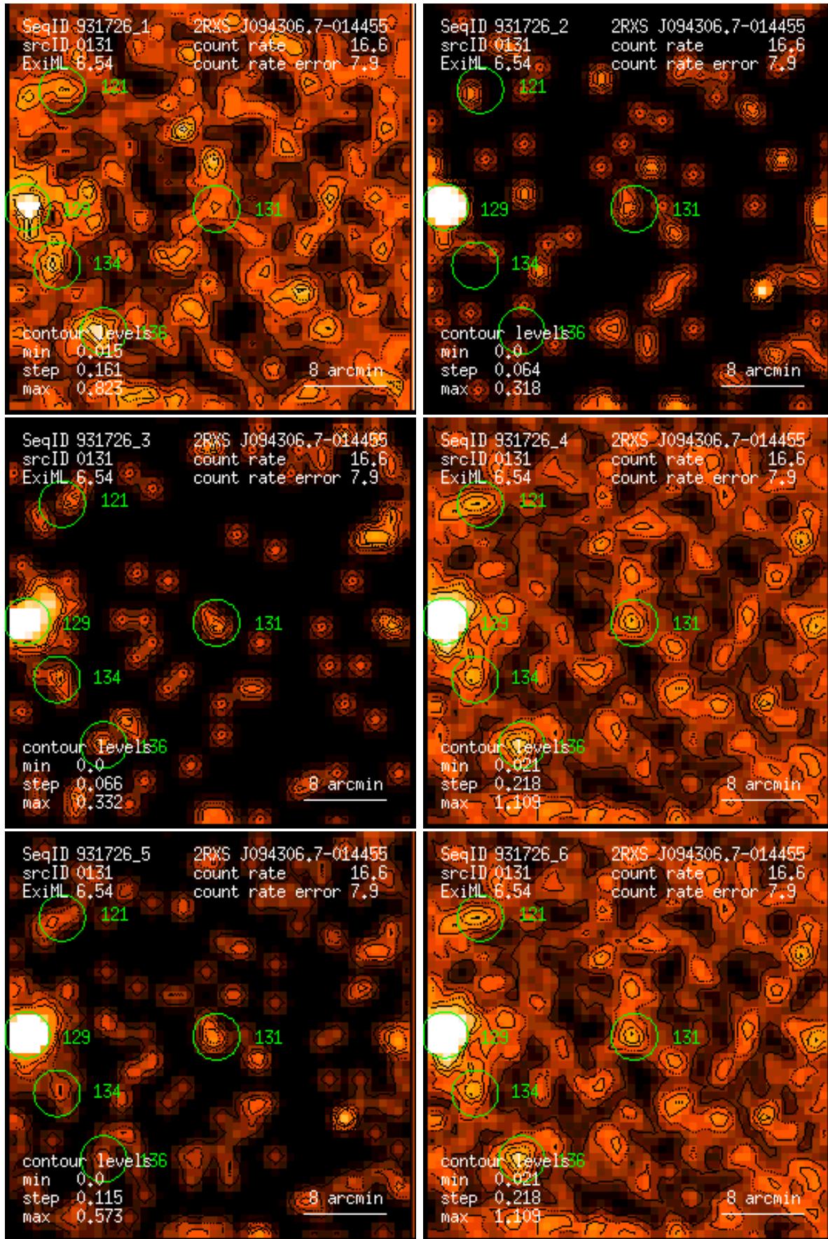
Figure 131: RASS 931726: detection 0131: band rate images, Gaussian filter: (1) PSPC channels 11 – 41, (2) 52 – 90, (3) 91 – 201, (4) 11 – 235, (5) 52 – 201, (6) 11 – 201. Broad band rates in counts/ks. Band rate contour levels in counts/ks/arcmin 2 .
