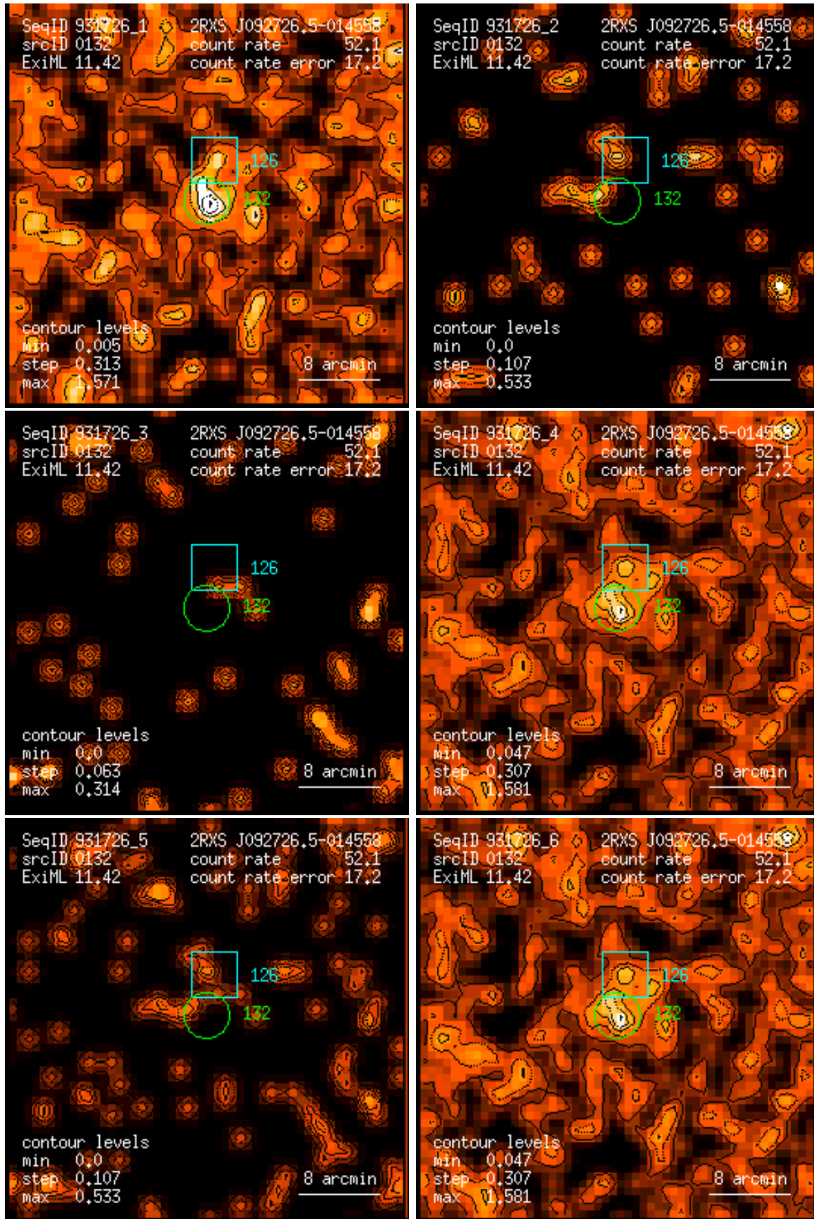
Figure 132: RASS 931726: detection 0132: band rate images, Gaussian filter: (1) PSPC channels 11 – 41, (2) 52 – 90, (3) 91 – 201, (4) 11 – 235, (5) 52 – 201, (6) 11 – 201. Broad band rates in counts/ks. Band rate contour levels in counts/ks/arcmin 2 .
