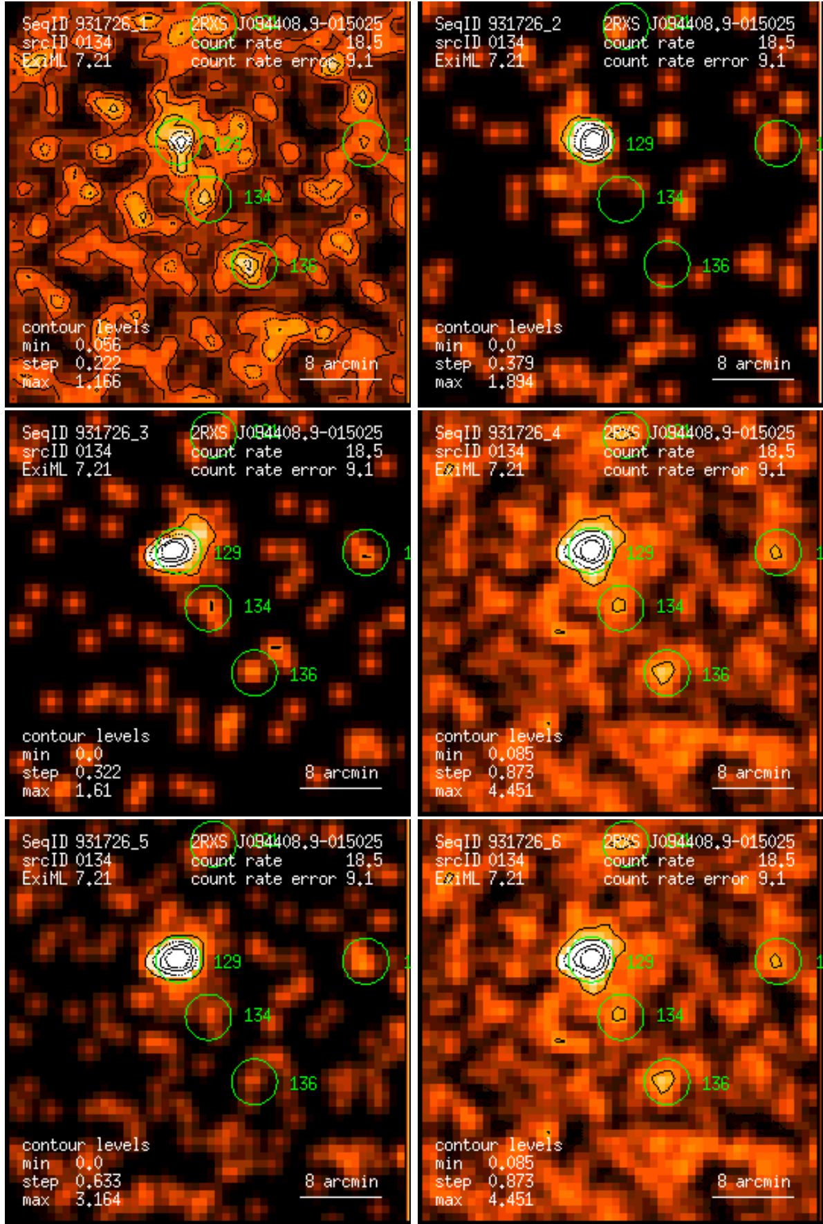
Figure 134: RASS 931726: detection 0134: band rate images, Gaussian filter: (1) PSPC channels 11 – 41, (2) 52 – 90, (3) 91 – 201, (4) 11 – 235, (5) 52 – 201, (6) 11 – 201. Broad band rates in counts/ks. Band rate contour levels in counts/ks/arcmin 2 .
