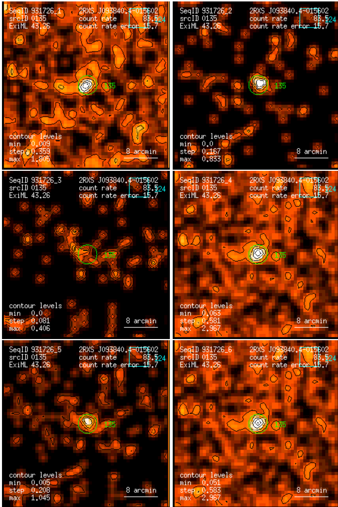
Figure 135: RASS 931726: detection 0135: band rate images, Gaussian filter: (1) PSPC channels 11 – 41, (2) 52 – 90, (3) 91 – 201, (4) 11 – 235, (5) 52 – 201, (6) 11 – 201. Broad band rates in counts/ks. Band rate contour levels in counts/ks/arcmin 2 .
