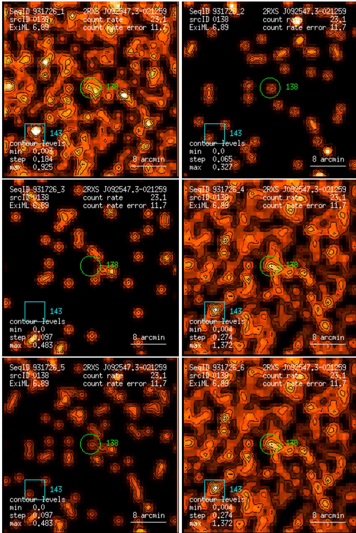
Figure 138: RASS 931726: detection 0138: band rate images, Gaussian filter: (1) PSPC channels 11 – 41, (2) 52 – 90, (3) 91 – 201, (4) 11 – 235, (5) 52 – 201, (6) 11 – 201. Broad band rates in counts/ks. Band rate contour levels in counts/ks/arcmin 2 .
