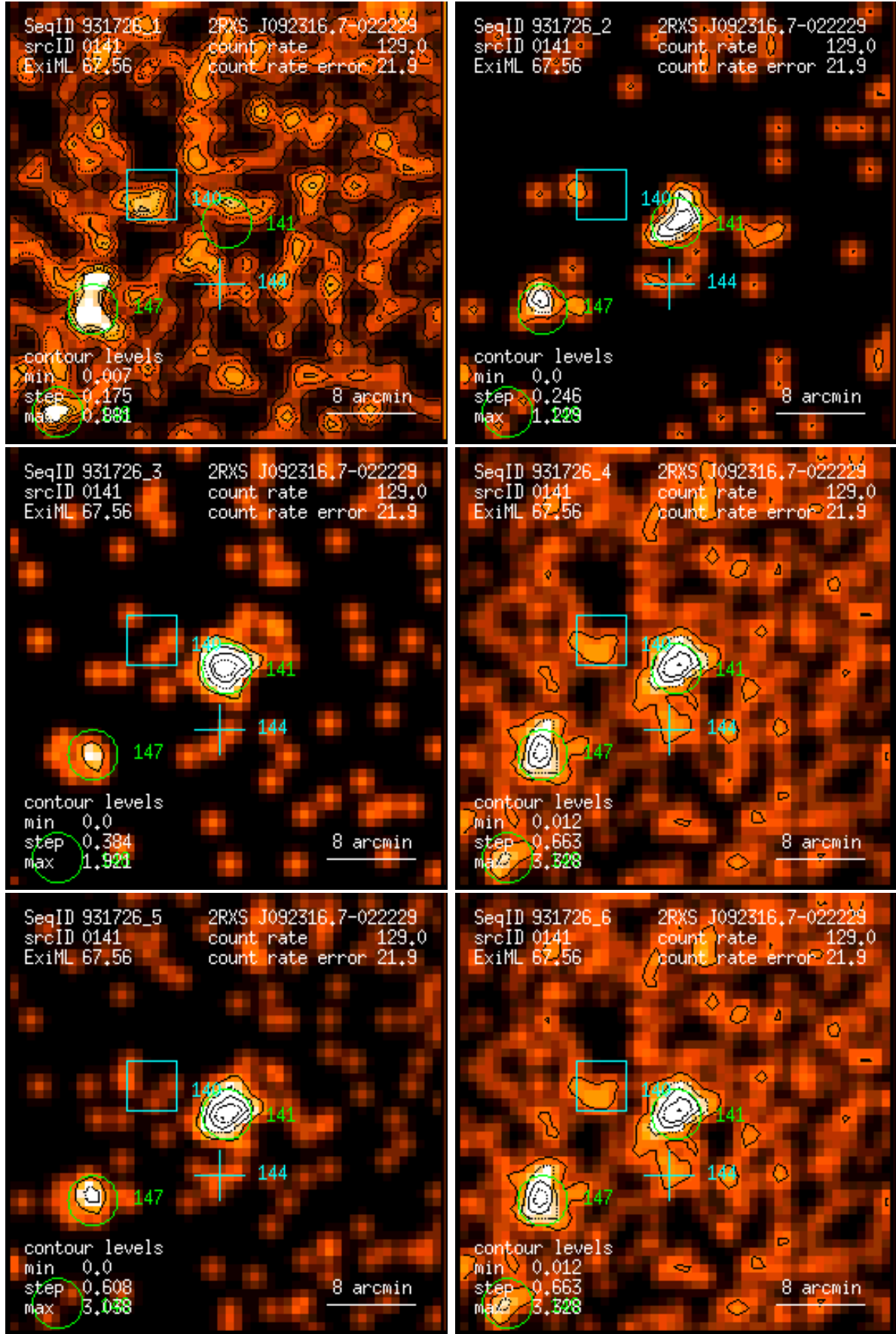
Figure 141: RASS 931726: detection 0141: band rate images, Gaussian filter: (1) PSPC channels 11 – 41, (2) 52 – 90, (3) 91 – 201, (4) 11 – 235, (5) 52 – 201, (6) 11 – 201. Broad band rates in counts/ks. Band rate contour levels in counts/ks/arcmin 2 .
