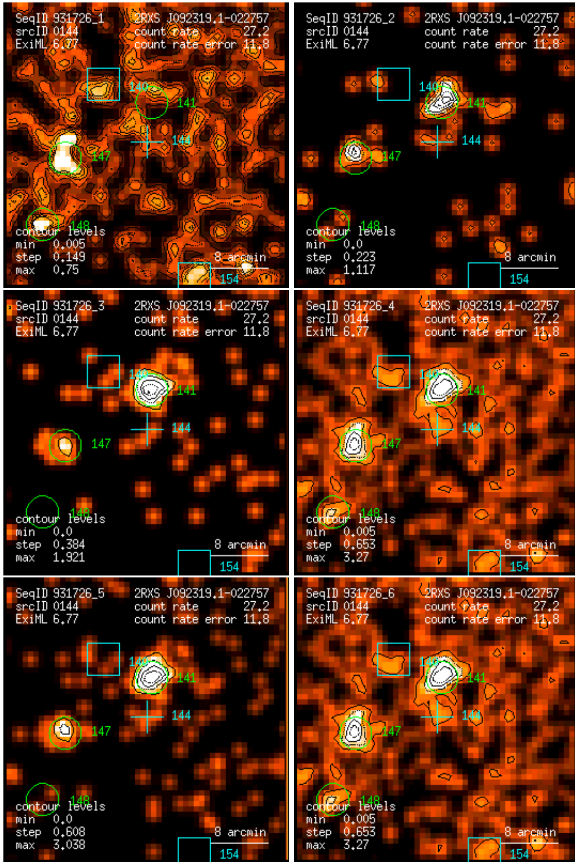
Figure 144: RASS 931726: detection 0144: band rate images, Gaussian filter: (1) PSPC channels 11 – 41, (2) 52 – 90, (3) 91 – 201, (4) 11 – 235, (5) 52 – 201, (6) 11 – 201. Broad band rates in counts/ks. Band rate contour levels in counts/ks/arcmin 2 .
