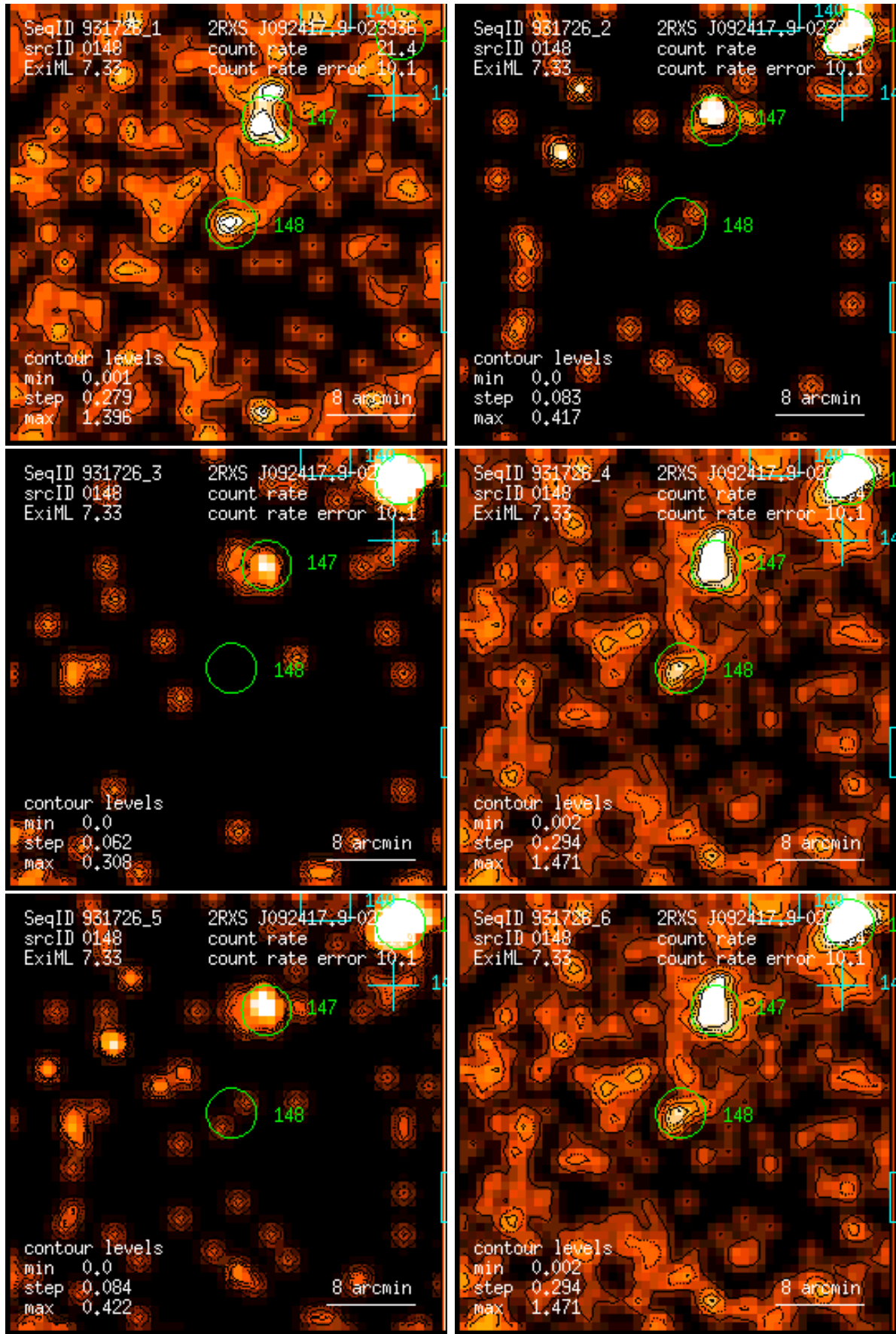
Figure 148: RASS 931726: detection 0148: band rate images, Gaussian filter: (1) PSPC channels 11 – 41, (2) 52 – 90, (3) 91 – 201, (4) 11 – 235, (5) 52 – 201, (6) 11 – 201. Broad band rates in counts/ks. Band rate contour levels in counts/ks/arcmin 2 .
