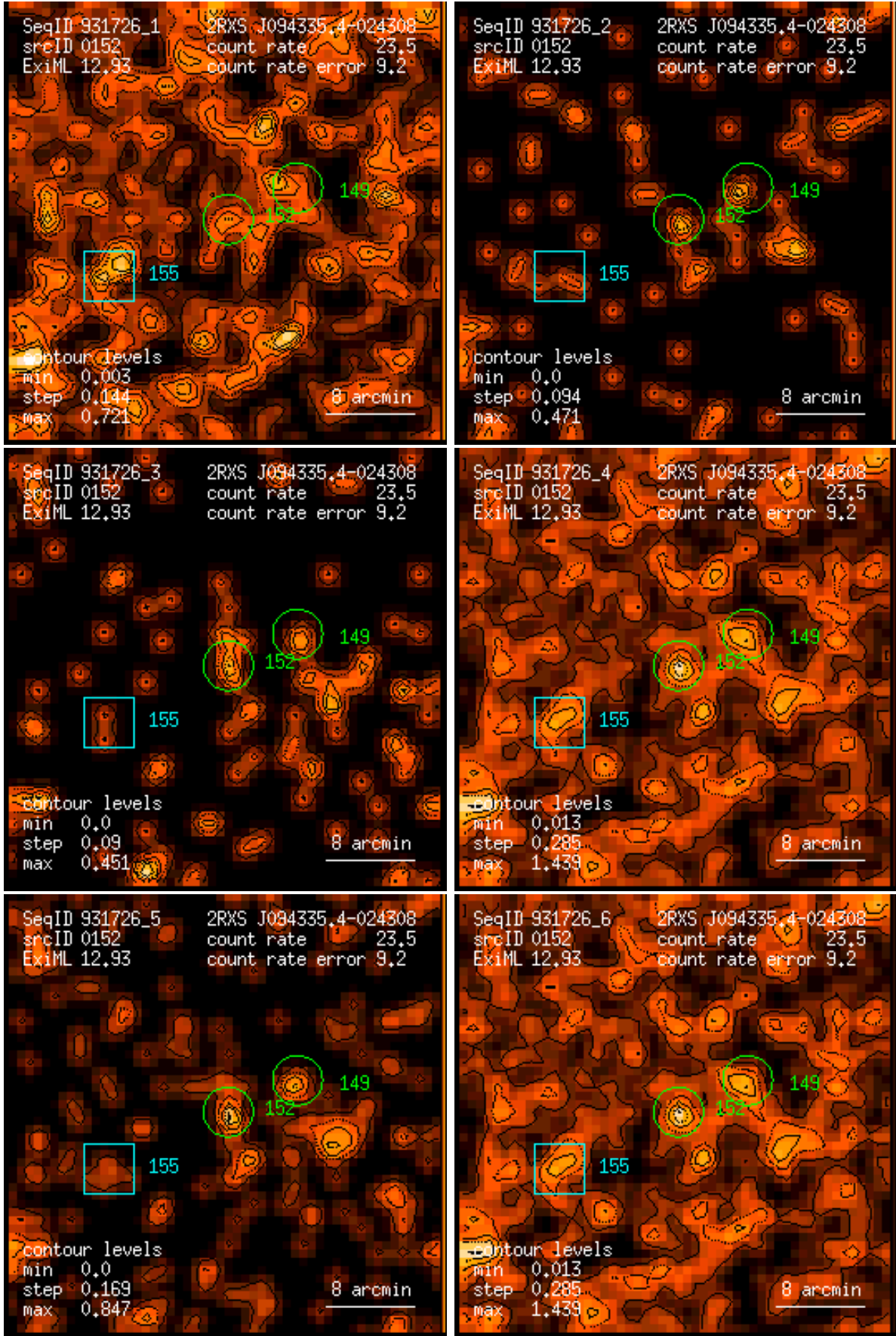
Figure 152: RASS 931726: detection 0152: band rate images, Gaussian filter: (1) PSPC channels 11 – 41, (2) 52 – 90, (3) 91 – 201, (4) 11 – 235, (5) 52 – 201, (6) 11 – 201. Broad band rates in counts/ks. Band rate contour levels in counts/ks/arcmin 2 .
