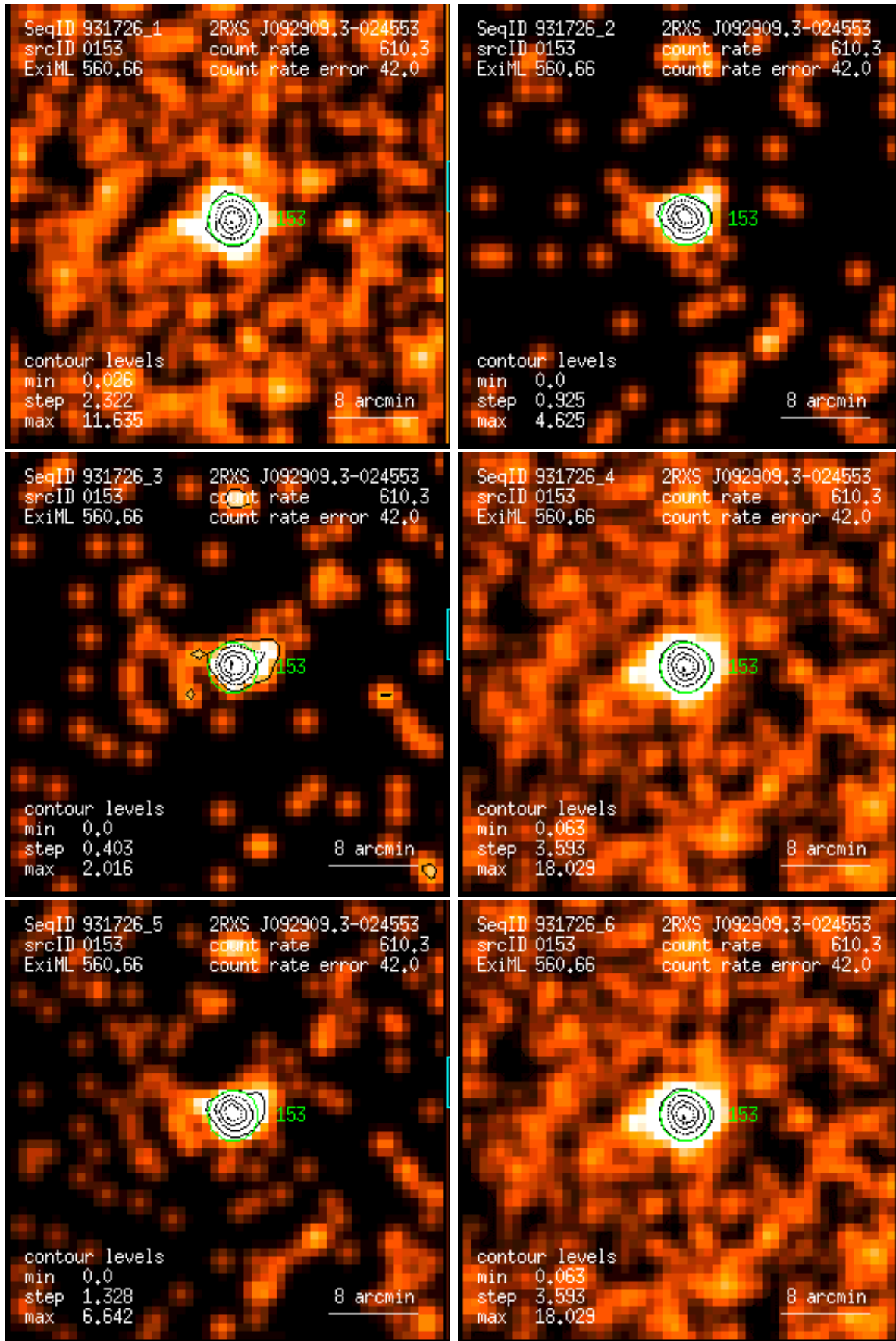
Figure 153: RASS 931726: detection 0153: band rate images, Gaussian filter: (1) PSPC channels 11 – 41, (2) 52 – 90, (3) 91 – 201, (4) 11 – 235, (5) 52 – 201, (6) 11 – 201. Broad band rates in counts/ks. Band rate contour levels in counts/ks/arcmin 2 .
